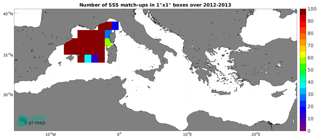
Figure 4: Number of SSS match-ups between Surface drifters SSS and the SMOS SSS L3 v335 - Monthly - 25 km (CATDS-CPDC) SSS product for the Mediterranean Sea Pi-MEP region over 1^\circ \times 1^\circ boxes and for the full satellite product period.
