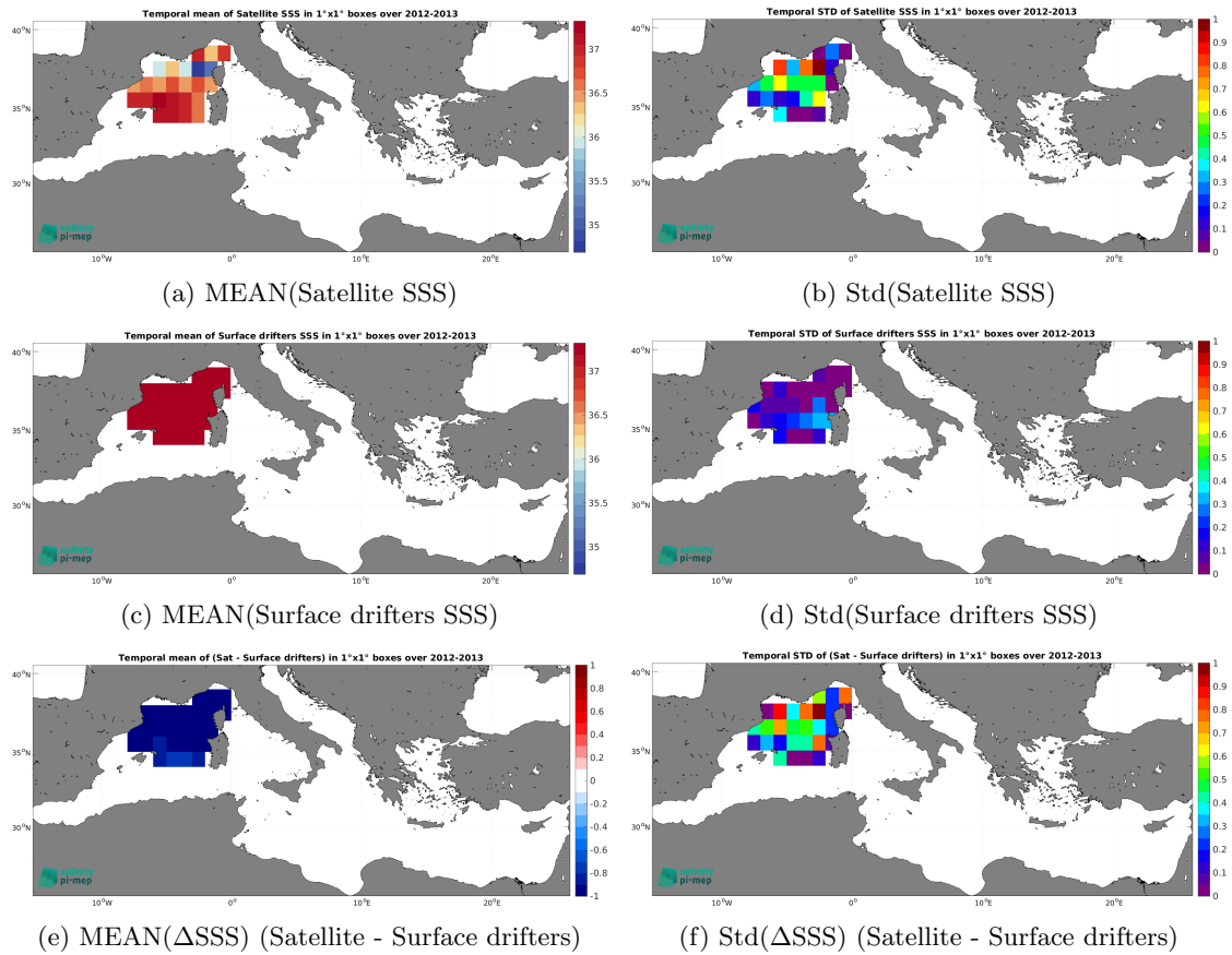
Figure 6: Temporal mean (left) and Std (right) of SSS from SMOS SSS L3 v335 - Monthly - 25 km (CATDS-CPDC) (top), Surface drifters (middle), and of \Delta SSS (Satellite - Surface drifters). Only match-up pairs are used to generate these maps.
