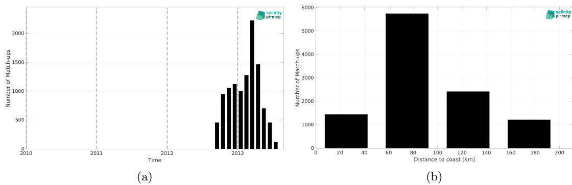
Figure 2: Number of match-ups between Surface drifters and SMOS SSS L3 v335 - Monthly - 25 km (CATDS-CPDC) SSS as a function of time (a) and as function of the distance to coast (b) over the Mediterranean Sea Pi-MEP region and for the full satellite product period.
