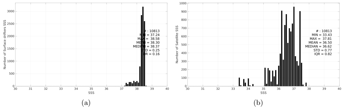
Figure 3: Histograms of SSS from Surface drifters (a) and SMOS SSS L3 v335 - Monthly - 25 km (CATDS-CPDC) (b) considering all match-up pairs per bins of 0.1 over the Mediterranean Sea Pi-MEP region and for the full satellite product period.
