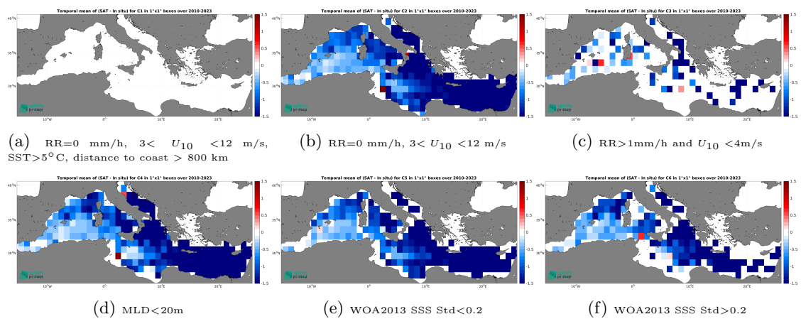
Figure 12: Temporal mean gridded over spatial boxes of size 1^\circ \times 1^\circ of \Delta SSS (SMOS SSS L3 v335 - Monthly - 25 km (CATDS-CPDC) - Argo) for 6 different subdatasets corresponding to:RR=0 mm/h, 3 < U_{10} < 12 m/s, SST >5^\circ\text{C} , distance to coast > 800 km (a), RR=0 mm/h, 3 < U_{10} < 12 m/s (b), RR >1 mm/h and U_{10} < 4 m/s (c),MLD <20 m (d),WOA2013 SSS Std <0.2 (e),WOA2013 SSS Std >0.2 (f).
