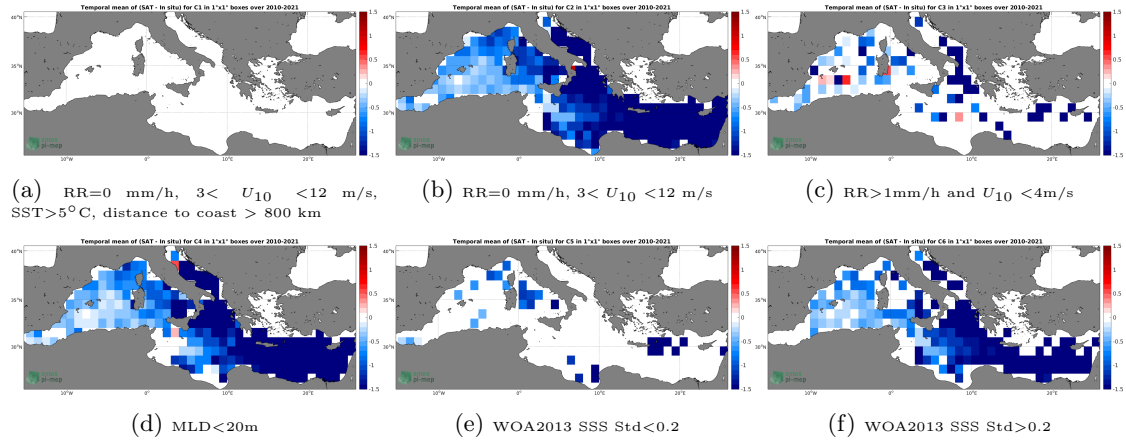
Figure 12: Temporal mean gridded over spatial boxes of size 1^\circ \times 1^\circ of \Delta SSS (SMOS SSS L3 v335 - Monthly - 25 km (CATDS-CPDC) - Argo) for 6 different subdatasets corresponding to: RR=0 mm/h, 3 < U_{10} < 12 m/s, SST > 5^\circ C , distance to coast > 800 km (a), RR=0 mm/h, 3 < U_{10} < 12 m/s (b), RR > 1 mm/h and U_{10} < 4 m/s (c), MLD < 20 m (d), WOA2013 SSS Std < 0.2 (e), WOA2013 SSS Std > 0.2 (f).
