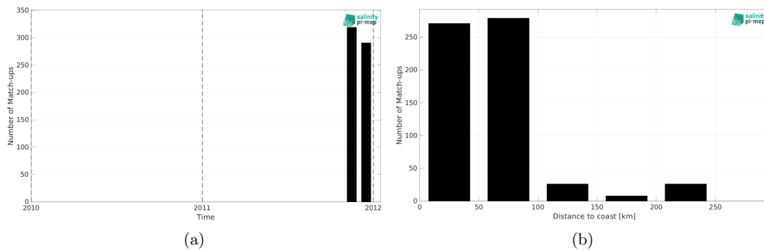
Figure 2: Number of match-ups between TSG (SAMOS) and SMOS SSS L3 v335 - 10 Days - 25 km (CATDS-CPDC) SSS as a function of time (a) and as function of the distance to coast (b) over the Mediterranean Sea Pi-MEP region and for the full satellite product period.
