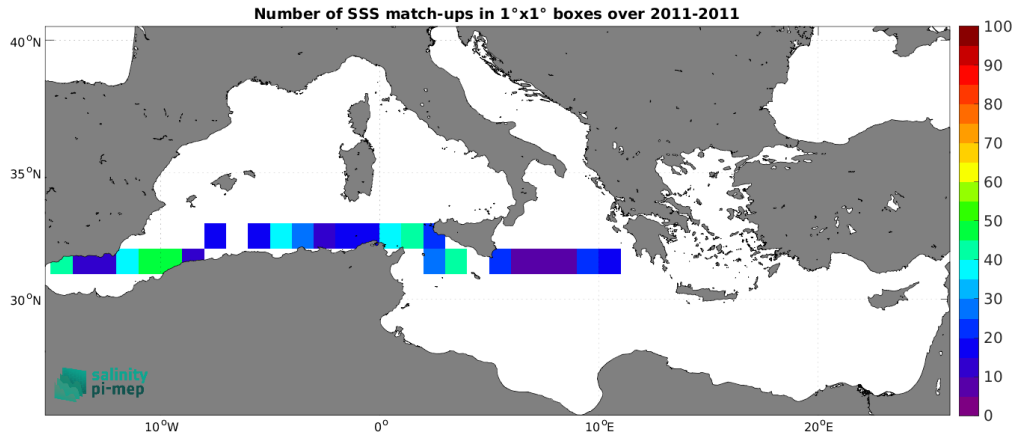
Figure 5: Number of SSS match-ups between TSG (SAMOS) SSS and the SMOS SSS L3 v335 - 10 Days - 25 km (CATDS-CPDC) SSS product for the Mediterranean Sea Pi-MEP region over 1^\circ \times 1^\circ boxes and for the full satellite product period.
