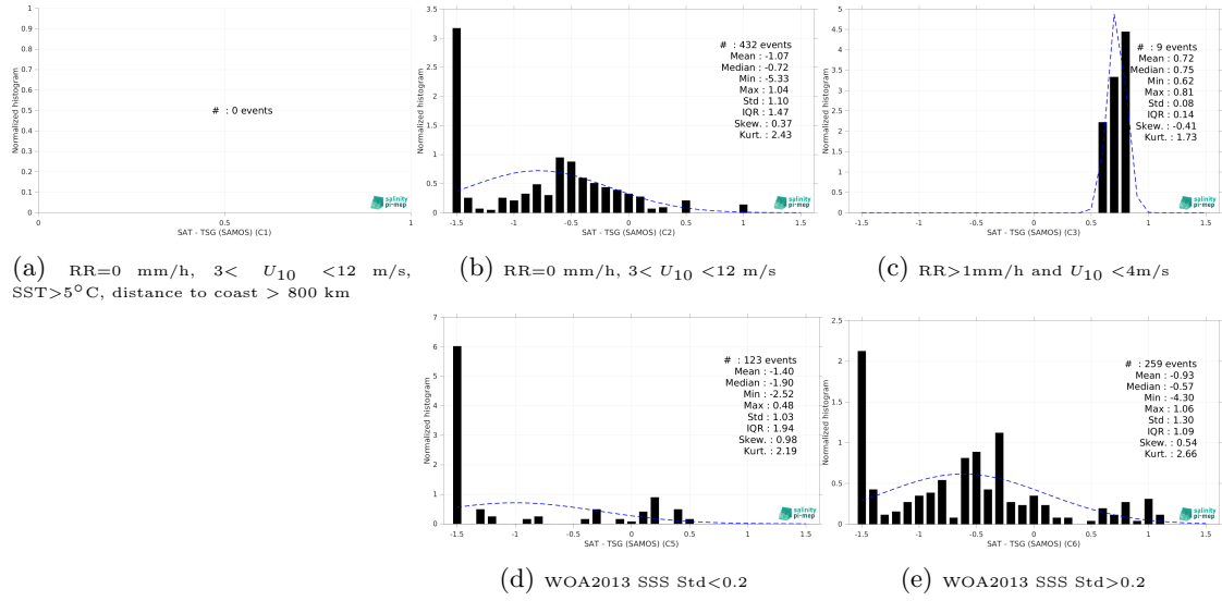
Figure 15: Normalized histogram of \Delta SSS (SMOS SSS L3 v335 - 10 Days - 25 km (CATDS-CPDC) - TSG (SAMOS)) for 5 different subdatasets corresponding to: RR=0 mm/h, 3 < U_{10} < 12 m/s, SST > 5°C, distance to coast > 800 km (a), RR=0 mm/h, 3 < U_{10} < 12 m/s (b), RR > 1mm/h and U_{10} < 4 m/s (c), WOA2013 SSS Std < 0.2 (d), WOA2013 SSS Std > 0.2 (e).
