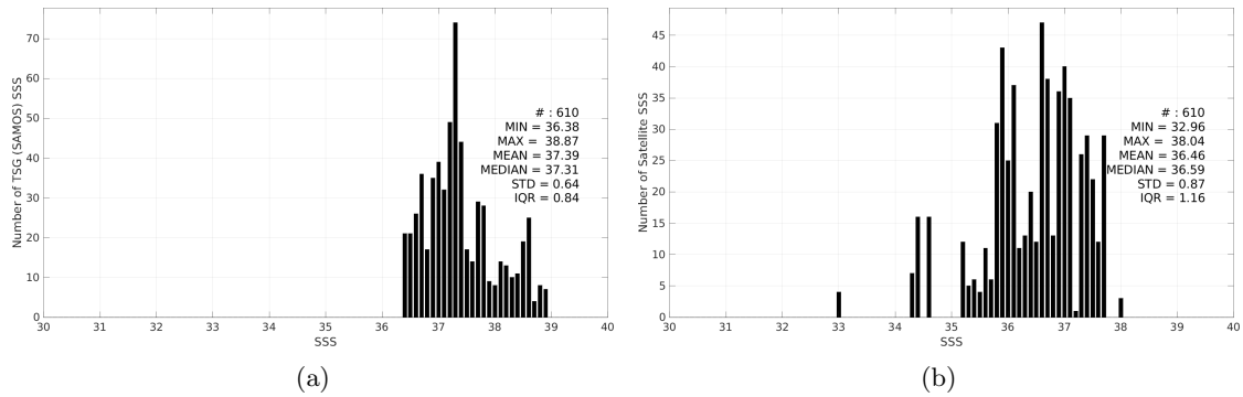
Figure 3: Histograms of SSS from TSG (SAMOS) (a) and SMOS SSS L3 v335 - 10 Days - 25 km (CATDS-CPDC) (b) considering all match-up pairs per bins of 0.1 over the Mediterranean Sea Pi-MEP region and for the full satellite product period.
