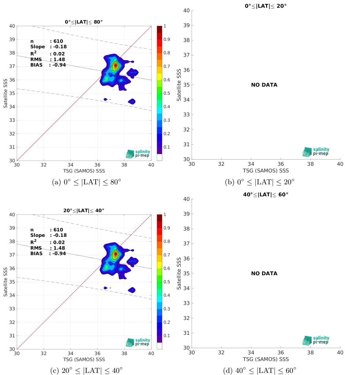
Figure 10: Contour maps of the concentration of SMOS SSS L3 v335 - 10 Days - 25 km (CATDS-CPDC) SSS (y-axis) versus TSG (SAMOS) SSS (x-axis) at match-up pairs for different latitude bands. For each plot, the red line shows x=y . The black thin and dashed lines indicate a linear fit through the data cloud and the \pm 95\% confidence levels, respectively. The number match-up pairs n , the slope and R^2 coefficient of the linear fit, the root mean square (RMS) and the mean bias between satellite and in situ data are indicated for each latitude band in each plots.
