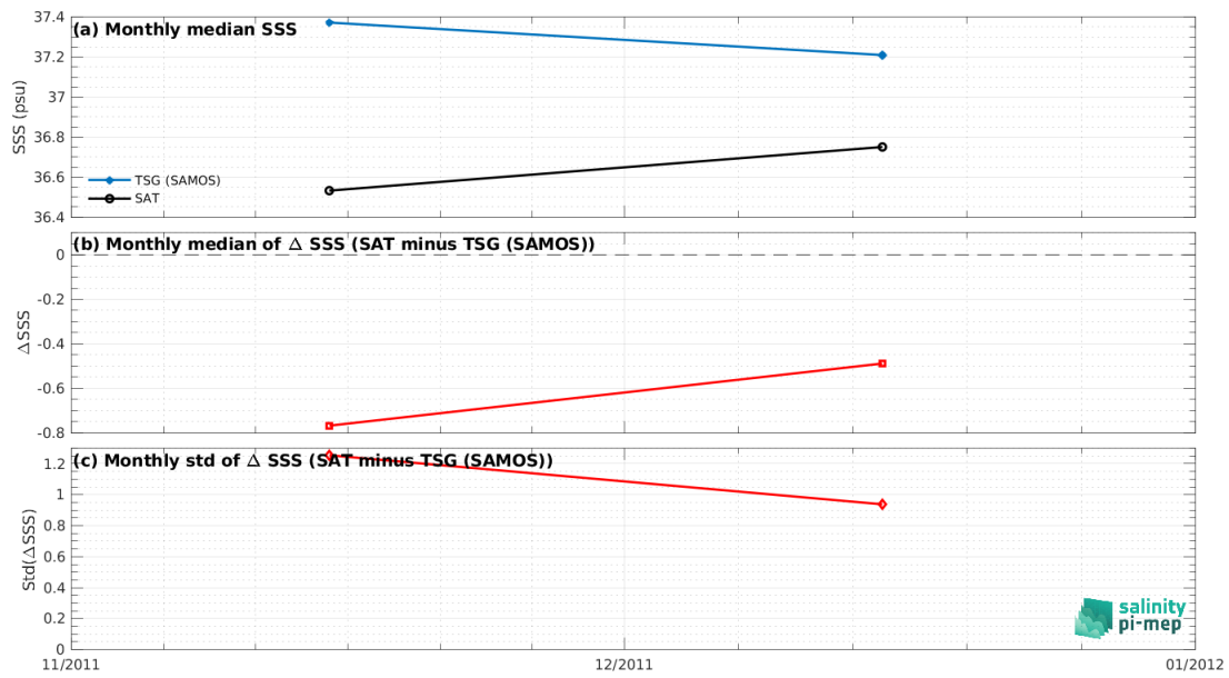
Figure 8: Time series of the monthly median SSS (top), median of \Delta SSS (Satellite - TSG (SAMOS)) and Std of \Delta SSS (Satellite - TSG (SAMOS)) over the Mediterranean Sea Pi-MEP region considering all match-ups collected by the Pi-MEP.
