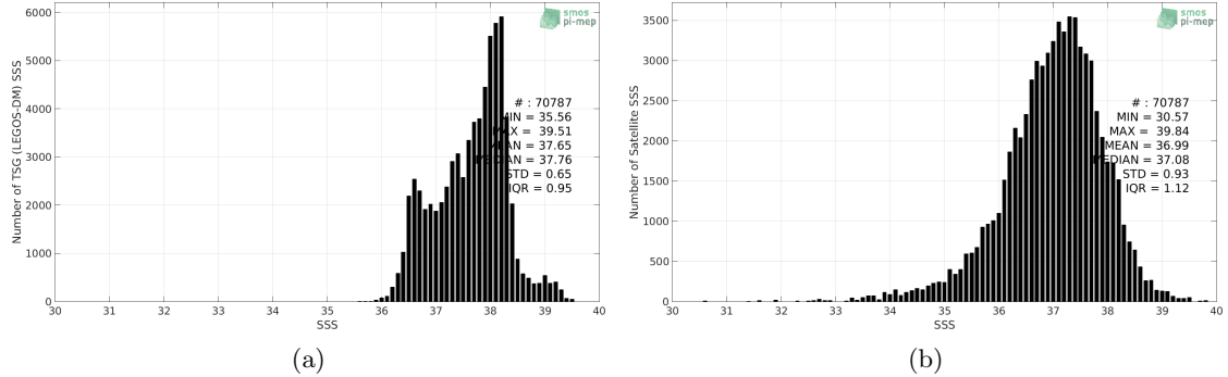
Figure 2: Histograms of SSS from TSG (LEGOS-DM) (a) and SMOS SSS L3 v335 - 10 Days - 25 km (CATDS-CPDC) (b) considering all match-up pairs per bins of 0.1 over the Mediterranean Sea Pi-MEP region and for the full satellite product period.
