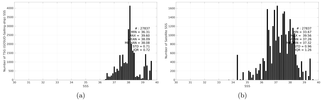
Figure 3: Histograms of SSS from TSG (GOSUD-Sailing-ship) (a) and SMOS SSS L3 v335 - 10 Days - 25 km (CATDS-CPDC) (b) considering all match-up pairs per bins of 0.1 over the Mediterranean Sea Pi-MEP region and for the full satellite product period.
