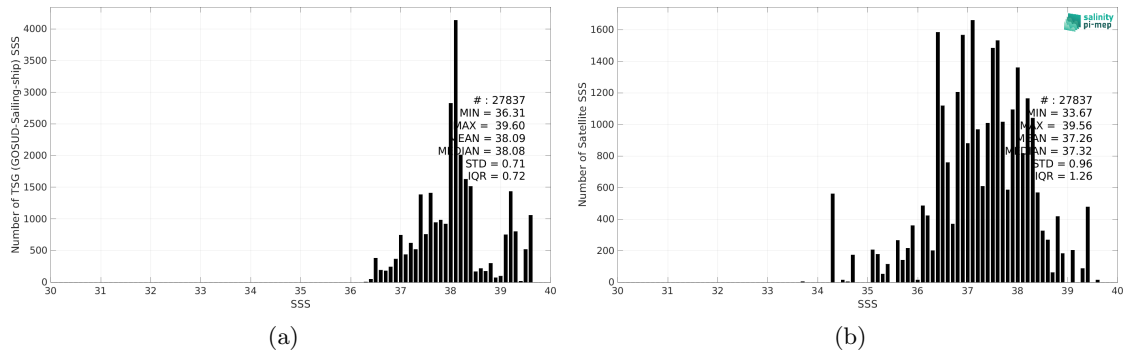
Figure 2: Histograms of SSS from TSG (GOSUD-Sailing-ship) (a) and SMOS SSS L3 v335 - 10 Days - 25 km (CATDS-CPDC) (b) considering all match-up pairs per bins of 0.1 over the Mediterranean Sea Pi-MEP region and for the full satellite product period.
