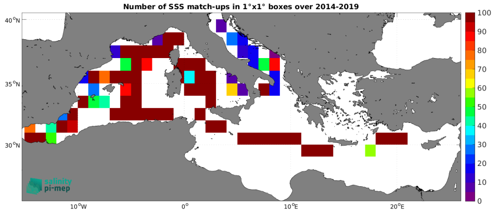
Figure 4: Number of SSS match-ups between TSG (GOSUD-Sailing-ship) SSS and the SMOS SSS L3 v335 - 10 Days - 25 km (CATDS-CPDC) SSS product for the Mediterranean Sea Pi-MEP region over 1^\circ \times 1^\circ boxes and for the full satellite product period.
