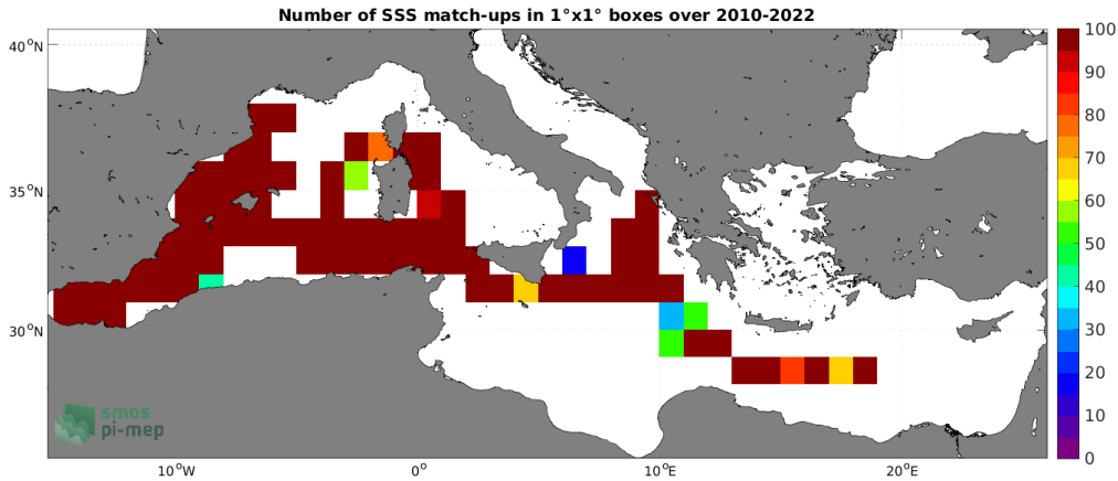
Figure 4: Number of SSS match-ups between TSG (CSIC-UTM) SSS and the SMOS SSS L3 v335 - 10 Days - 25 km (CATDS-CPDC) SSS product for the Mediterranean Sea Pi-MEP region over 1^\circ \times 1^\circ boxes and for the full satellite product period.
