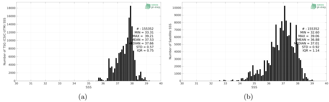
Figure 2: Histograms of SSS from TSG (CSIC-UTM) (a) and SMOS SSS L3 v335 - 10 Days - 25 km (CATDS-CPDC) (b) considering all match-up pairs per bins of 0.1 over the Mediterranean Sea Pi-MEP region and for the full satellite product period.
