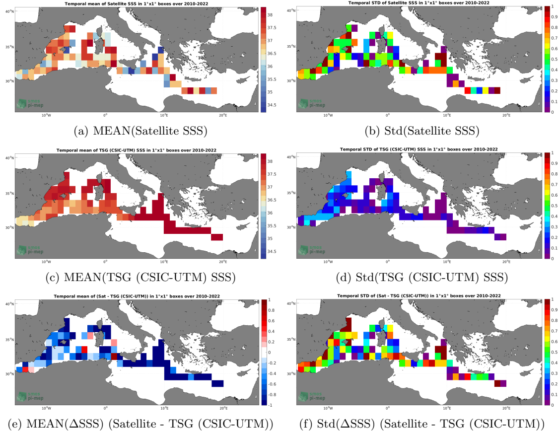
Figure 6: Temporal mean (left) and Std (right) of SSS from SMOS SSS L3 v335 - 10 Days - 25 km (CATDS-CPDC) (top), TSG (CSIC-UTM) (middle), and of \Delta\text{SSS} (Satellite - TSG (CSIC-UTM)). Only match-up pairs are used to generate these maps.
