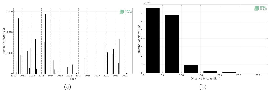
Figure 1: Number of match-ups between TSG (CSIC-UTM) and SMOS SSS L3 v335 - 10 Days - 25 km (CATDS-CPDC) SSS as a function of time (a) and as function of the distance to coast (b) over the Mediterranean Sea Pi-MEP region and for the full satellite product period.
