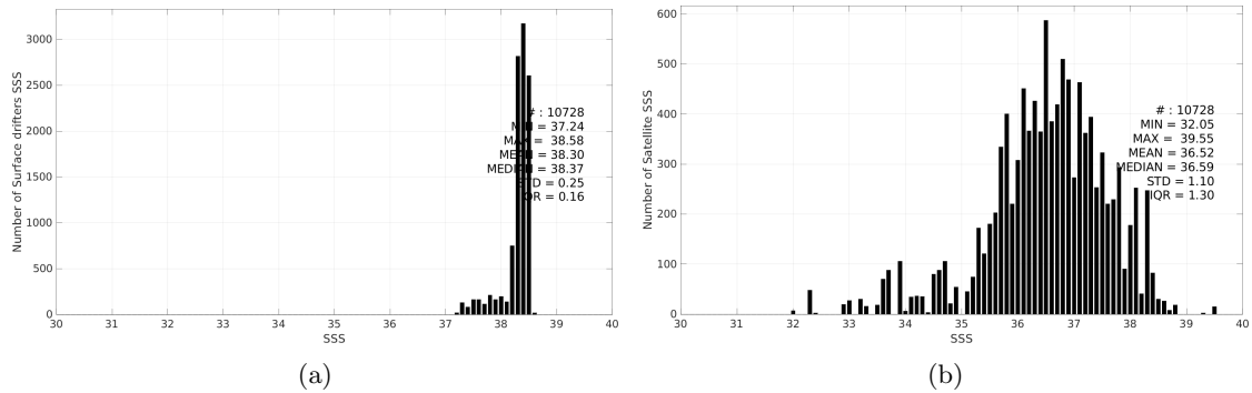
Figure 3: Histograms of SSS from Surface drifters (a) and SMOS SSS L3 v335 - 10 Days - 25 km (CATDS-CPDC) (b) considering all match-up pairs per bins of 0.1 over the Mediterranean Sea Pi-MEP region and for the full satellite product period.
