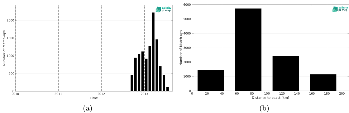
Figure 2: Number of match-ups between Surface drifters and SMOS SSS L3 v335 - 10 Days - 25 km (CATDS-CPDC) SSS as a function of time (a) and as function of the distance to coast (b) over the Mediterranean Sea Pi-MEP region and for the full satellite product period.
