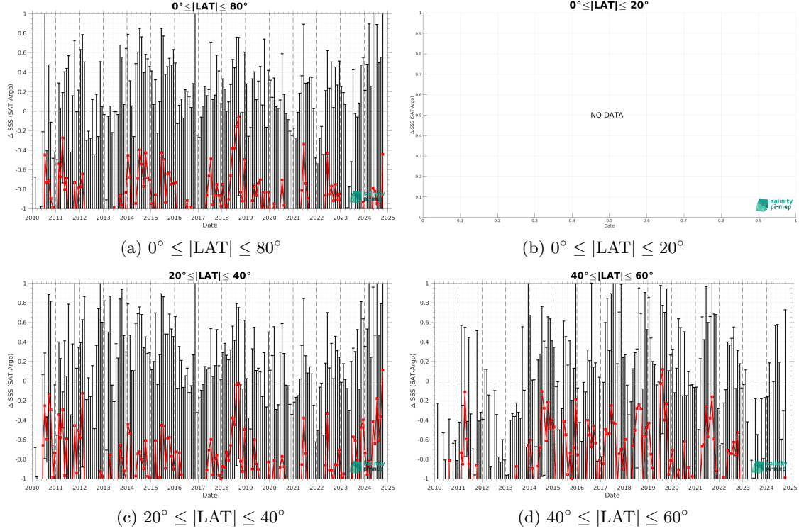
Figure 11: Monthly median (red curves) of \Delta SSS (Satellite - Argo) and \pm 1 Std (black vertical thick bars) as function of time for all the collected Pi-MEP match-up pairs estimated over the Mediterranean Sea Pi-MEP region and for the full satellite product period are shown for different latitude bands: (a) 80°S-80°N, (b) 20°S-20°N, (c) 40°S-20°S and 20°N-40°N and (d) 60°S-40°S and 40°N-60°N.
