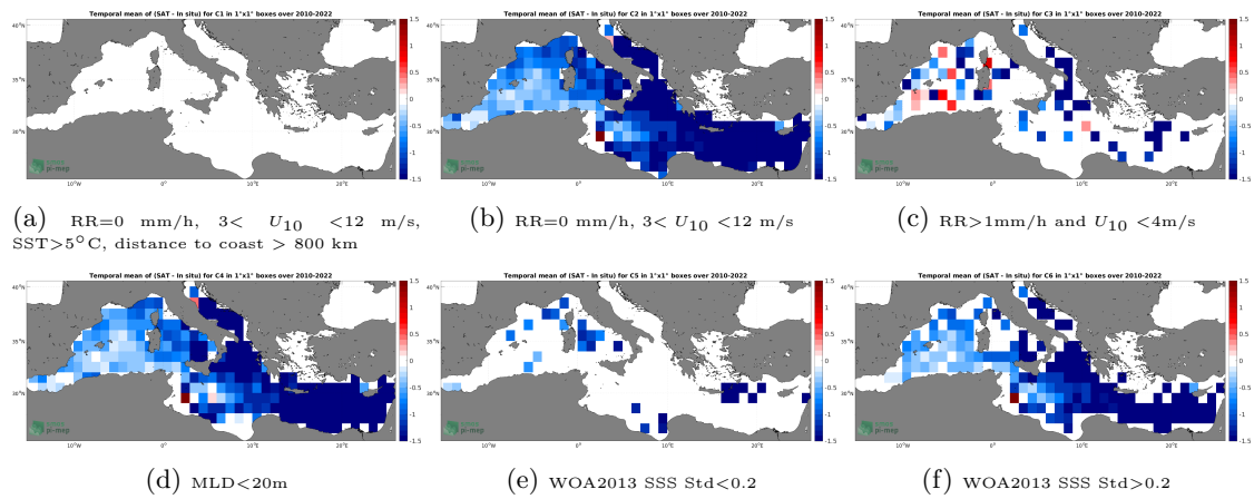
Figure 12: Temporal mean gridded over spatial boxes of size 1^\circ \times 1^\circ of \Delta SSS (SMOS SSS L3 v335 - 10 Days - 25 km (CATDS-CPDC) - Argo) for 6 different subdatasets corresponding to:RR=0 mm/h, 3 < U_{10} < 12 m/s, SST >5^\circ C, distance to coast > 800 km (a), RR=0 mm/h, 3 < U_{10} < 12 m/s (b), RR >1 mm/h and U_{10} < 4 m/s (c),MLD <20 m (d),WOA2013 SSS Std <0.2 (e),WOA2013 SSS Std >0.2 (f).
