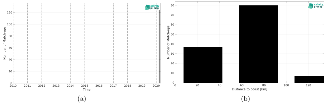
Figure 2: Number of match-ups between Saildrone and SMOS SSS L2Q v333 - 0.25 Deg (CATDS-CPDC) SSS as a function of time (a) and as function of the distance to coast (b) over the Mediterranean Sea Pi-MEP region and for the full satellite product period.
