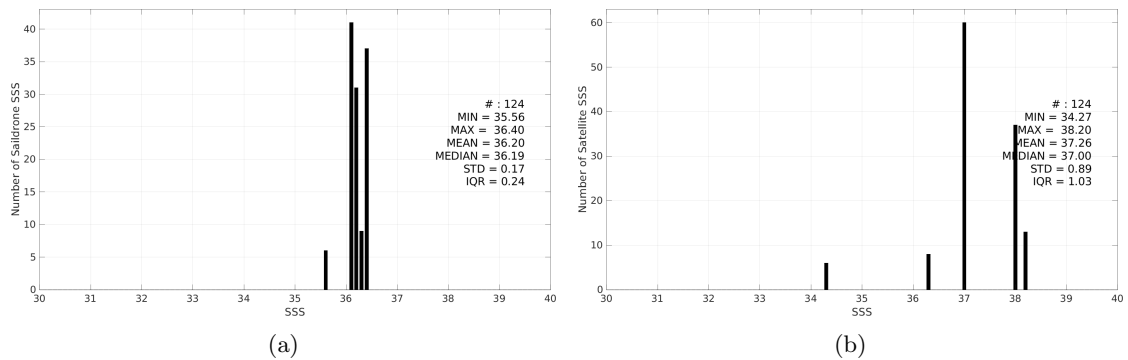
Figure 3: Histograms of SSS from Saildrone (a) and SMOS SSS L2Q v333 - 0.25 Deg (CATDS-CPDC) (b) considering all match-up pairs per bins of 0.1 over the Mediterranean Sea Pi-MEP region and for the full satellite product period.
