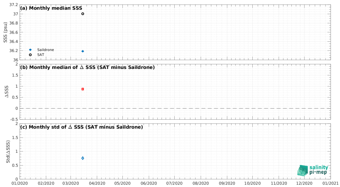
Figure 8: Time series of the monthly median SSS (top), median of \Delta SSS (Satellite - SAILDRONE) and Std of \Delta SSS (Satellite - SAILDRONE) over the Mediterranean Sea Pi-MEP region considering all match-ups collected by the Pi-MEP.
