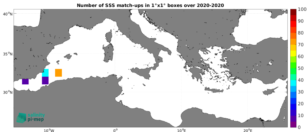
Figure 5: Number of SSS match-ups between Saildrone SSS and the SMOS SSS L2Q v333 - 0.25 Deg (CATDS-CPDC) SSS product for the Mediterranean Sea Pi-MEP region over 1^\circ \times 1^\circ boxes and for the full satellite product period.
