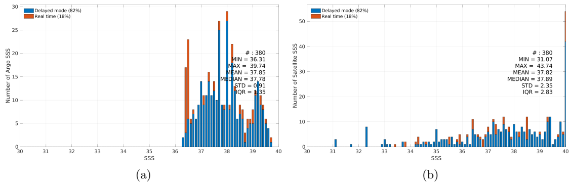
Figure 3: Histograms of SSS from Argo (a) and SMOS SSS L2Q v333 - 0.25 Deg (CATDS-CPDC) (b) considering all match-up pairs per bins of 0.1 over the Mediterranean Sea Pi-MEP region and for the full satellite product period.
