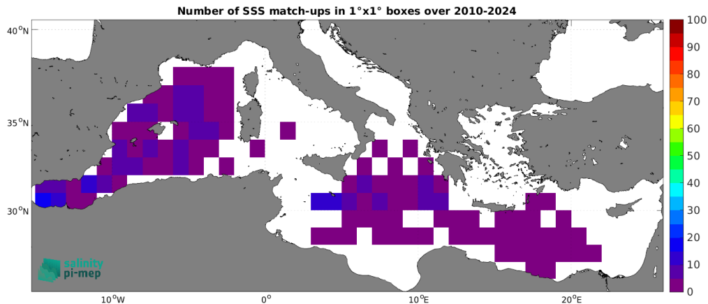
Figure 5: Number of SSS match-ups between Argo SSS and the SMOS SSS L2Q v333 - 0.25 Deg (CATDS-CPDC) SSS product for the Mediterranean Sea Pi-MEP region over 1^\circ \times 1^\circ boxes and for the full satellite product period.
