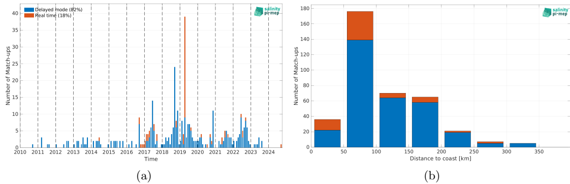
Figure 2: Number of match-ups between Argo and SMOS SSS L2Q v333 - 0.25 Deg (CATDS-CPDC) SSS as a function of time (a) and as function of the distance to coast (b) over the Mediterranean Sea Pi-MEP region and for the full satellite product period.
