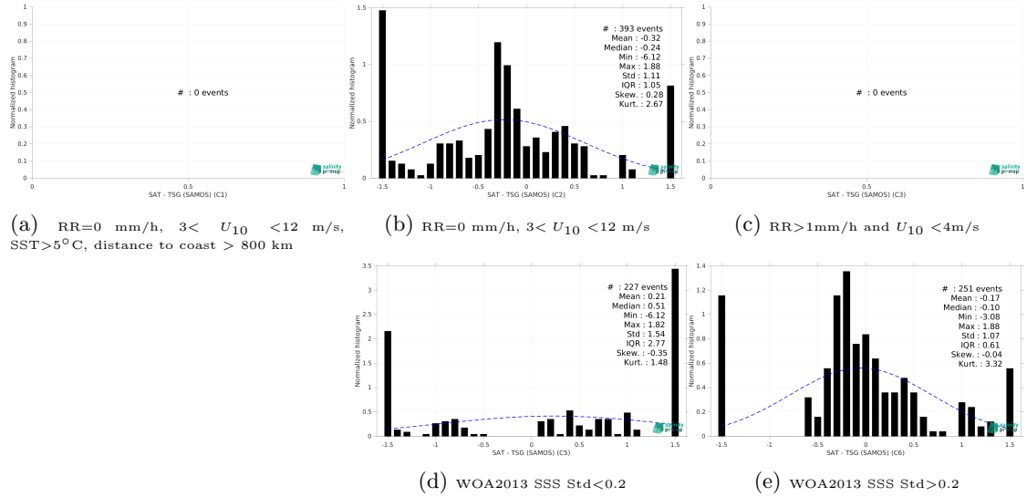
Figure 15: Normalized histogram of \Delta SSS (SMOS SSS L3 v332 - 9 Days (CATDS-CPDC) - TSG (SAMOS)) for 5 different subdatasets corresponding to: RR=0 mm/h, 3 < U_{10} < 12 m/s, SST>5°C, distance to coast > 800 km (a), RR=0 mm/h, 3 < U_{10} < 12 m/s (b), RR>1mm/h and U_{10} < 4 m/s (c), WOA2013 SSS Std<0.2 (d), WOA2013 SSS Std>0.2 (e).
