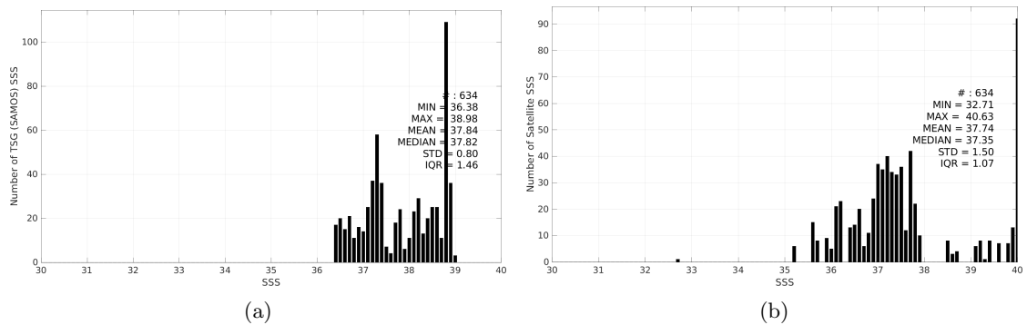
Figure 3: Histograms of SSS from TSG (SAMOS) (a) and SMOS SSS L3 v332 - 9 Days (CATDS-CPDC) (b) considering all match-up pairs per bins of 0.1 over the Mediterranean Sea Pi-MEP region and for the full satellite product period.
