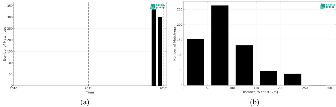
Figure 2: Number of match-ups between TSG (SAMOS) and SMOS SSS L3 v332 - 9 Days (CATDS-CPDC) SSS as a function of time (a) and as function of the distance to coast (b) over the Mediterranean Sea Pi-MEP region and for the full satellite product period.
