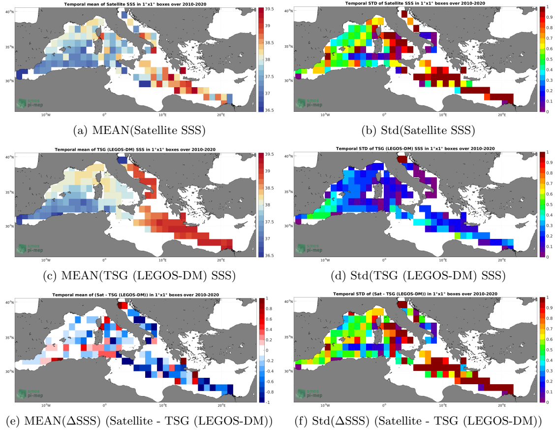
Figure 6: Temporal mean (left) and Std (right) of SSS from SMOS SSS L3 v332 - 9 Days (CATDS-CPDC) (top), TSG (LEGOS-DM) (middle), and of \Delta SSS (Satellite - TSG (LEGOS-DM)). Only match-up pairs are used to generate these maps.
