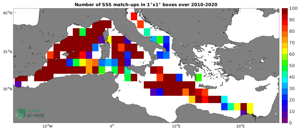
Figure 4: Number of SSS match-ups between TSG (LEGOS-DM) SSS and the SMOS SSS L3 v332 - 9 Days (CATDS-CPDC) SSS product for the Mediterranean Sea Pi-MEP region over 1^\circ \times 1^\circ boxes and for the full satellite product period.
