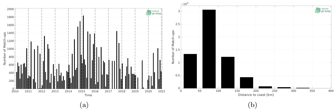
Figure 1: Number of match-ups between TSG (LEGOS-DM) and SMOS SSS L3 v332 - 9 Days (CATDS-CPDC) SSS as a function of time (a) and as function of the distance to coast (b) over the Mediterranean Sea Pi-MEP region and for the full satellite product period.
