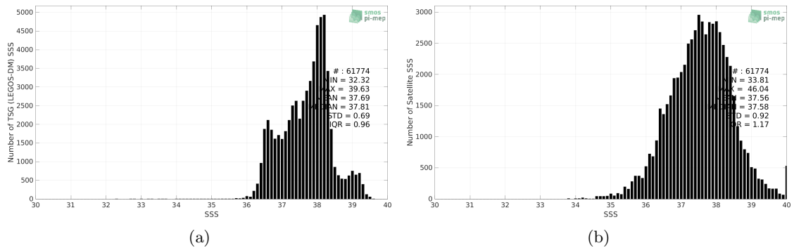
Figure 2: Histograms of SSS from TSG (LEGOS-DM) (a) and SMOS SSS L3 v332 - 9 Days (CATDS-CPDC) (b) considering all match-up pairs per bins of 0.1 over the Mediterranean Sea Pi-MEP region and for the full satellite product period.
