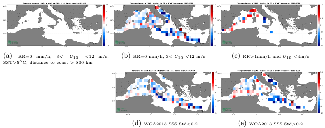
Figure 12: Temporal mean gridded over spatial boxes of size 1^\circ \times 1^\circ of \Delta SSS (SMOS SSS L3 v332 - 9 Days (CATDS-CPDC) - TSG (LEGOS-DM)) for 5 different subdatasets corresponding to:RR=0 mm/h, 3 < U_{10} < 12 m/s, SST >5^\circ C, distance to coast > 800 km (a), RR=0 mm/h, 3 < U_{10} < 12 m/s (b), RR >1 mm/h and U_{10} < 4 m/s (c), WOA2013 SSS Std <0.2 (d), WOA2013 SSS Std >0.2 (e).
