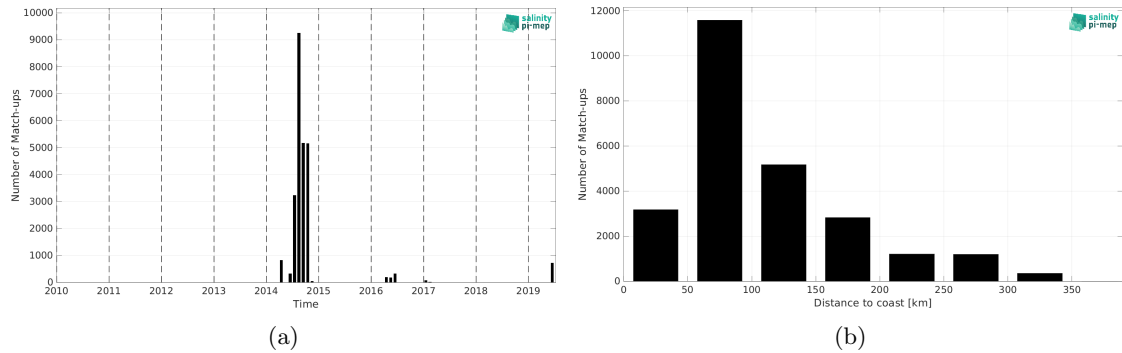
Figure 2: Number of match-ups between TSG (GOSUD-Sailing-ship) and SMOS SSS L3 v332 - 9 Days (CATDS-CPDC) SSS as a function of time (a) and as function of the distance to coast (b) over the Mediterranean Sea Pi-MEP region and for the full satellite product period.
