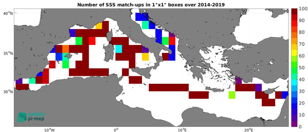
Figure 5: Number of SSS match-ups between TSG (GOSUD-Sailing-ship) SSS and the SMOS SSS L3 v332 - 9 Days (CATDS-CPDC) SSS product for the Mediterranean Sea Pi-MEP region over 1^\circ \times 1^\circ boxes and for the full satellite product period.
