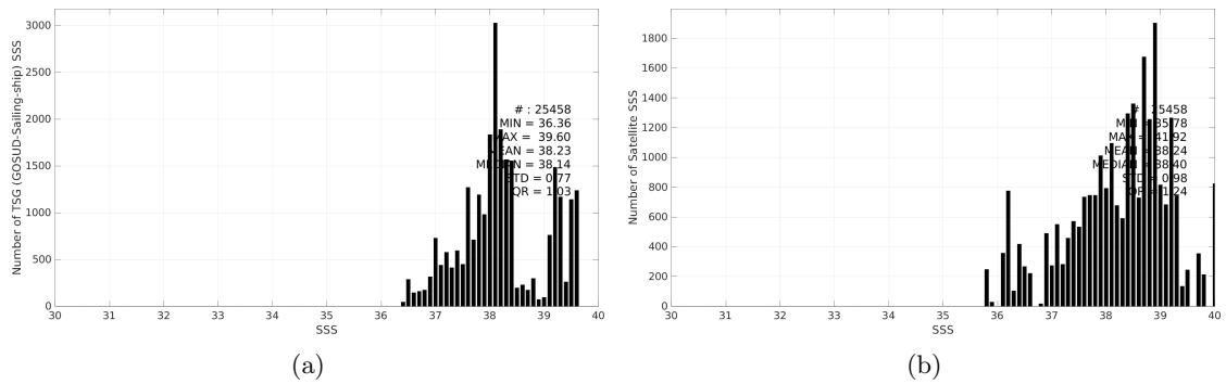
Figure 3: Histograms of SSS from TSG (GOSUD-Sailing-ship) (a) and SMOS SSS L3 v332 - 9 Days (CATDS-CPDC) (b) considering all match-up pairs per bins of 0.1 over the Mediterranean Sea Pi-MEP region and for the full satellite product period.
