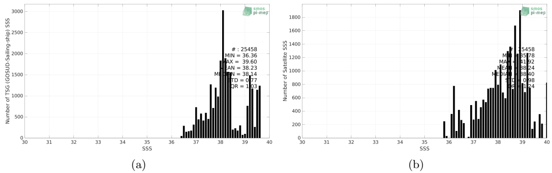
Figure 2: Histograms of SSS from TSG (GOSUD-Sailing-ship) (a) and SMOS SSS L3 v332 - 9 Days (CATDS-CPDC) (b) considering all match-up pairs per bins of 0.1 over the Mediterranean Sea Pi-MEP region and for the full satellite product period.
