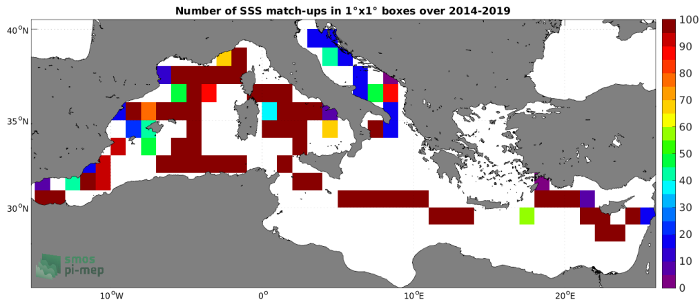
Figure 4: Number of SSS match-ups between TSG (GOSUD-Sailing-ship) SSS and the SMOS SSS L3 v332 - 9 Days (CATDS-CPDC) SSS product for the Mediterranean Sea Pi-MEP region over 1^\circ \times 1^\circ boxes and for the full satellite product period.
