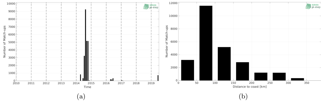
Figure 1: Number of match-ups between TSG (GOSUD-Sailing-ship) and SMOS SSS L3 v332 - 9 Days (CATDS-CPDC) SSS as a function of time (a) and as function of the distance to coast (b) over the Mediterranean Sea Pi-MEP region and for the full satellite product period.
