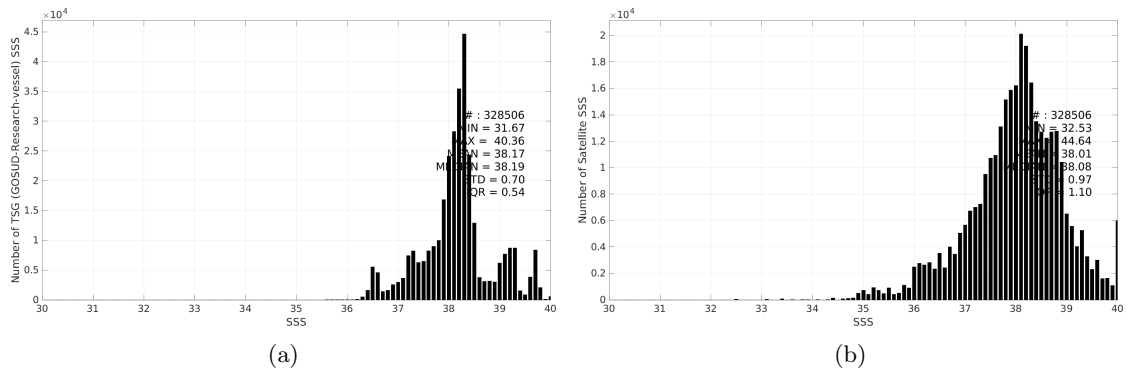
Figure 3: Histograms of SSS from TSG (GOSUD-Research-vessel) (a) and SMOS SSS L3 v332 - 9 Days (CATDS-CPDC) (b) considering all match-up pairs per bins of 0.1 over the Mediterranean Sea Pi-MEP region and for the full satellite product period.
