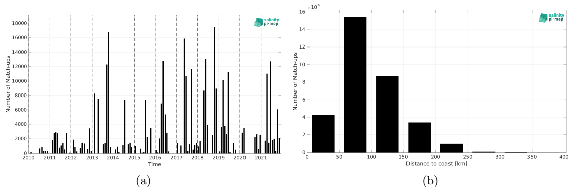
Figure 2: Number of match-ups between TSG (GOSUD-Research-vessel) and SMOS SSS L3 v332 - 9 Days (CATDS-CPDC) SSS as a function of time (a) and as function of the distance to coast (b) over the Mediterranean Sea Pi-MEP region and for the full satellite product period.
