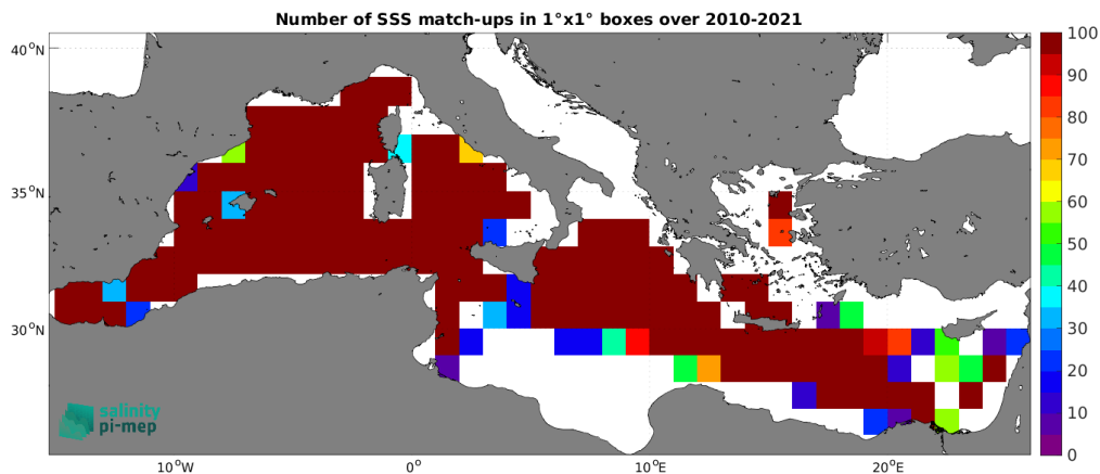
Figure 5: Number of SSS match-ups between TSG (GOSUD-Research-vessel) SSS and the SMOS SSS L3 v332 - 9 Days (CATDS-CPDC) SSS product for the Mediterranean Sea Pi-MEP region over 1^\circ \times 1^\circ boxes and for the full satellite product period.
