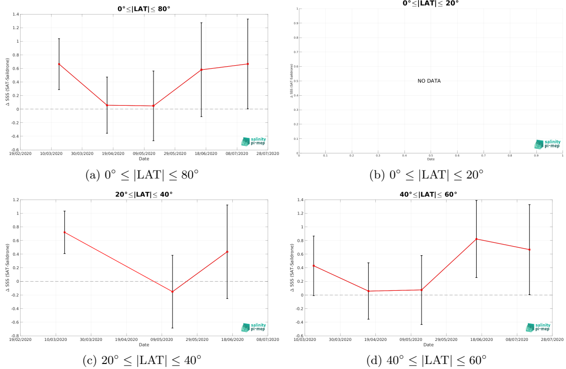
Figure 11: Monthly median (red curves) of \Delta\text{SSS} (Satellite - Saldrone) and \pm 1 Std (black vertical thick bars) as function of time for all the collected Pi-MEP match-up pairs estimated over the Mediterranean Sea Pi-MEP region and for the full satellite product period are shown for different latitude bands: (a) 80^{\circ}\text{S}-80^{\circ}\text{N} , (b) 20^{\circ}\text{S}-20^{\circ}\text{N} , (c) 40^{\circ}\text{S}-20^{\circ}\text{S} and 20^{\circ}\text{N}-40^{\circ}\text{N} and (d) 60^{\circ}\text{S}-40^{\circ}\text{S} and 40^{\circ}\text{N}-60^{\circ}\text{N} .
