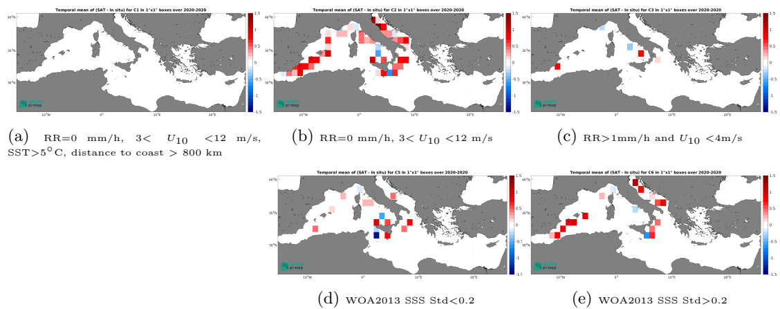
Figure 14: Temporal mean gridded over spatial boxes of size 1^\circ \times 1^\circ of \Delta\text{SSS} (SMOS SSS L3 v332 - 9 Days (CATDS-CPDC) - Sairdrone) for 5 different subdatasets corresponding to:RR=0 mm/h, 3 < U_{10} < 12 m/s, SST>5°C, distance to coast > 800 km (a), RR=0 mm/h, 3 < U_{10} < 12 m/s (b), RR>1mm/h and U_{10} < 4 m/s (c), WOA2013 SSS Std<0.2 (d), WOA2013 SSS Std>0.2 (e).
