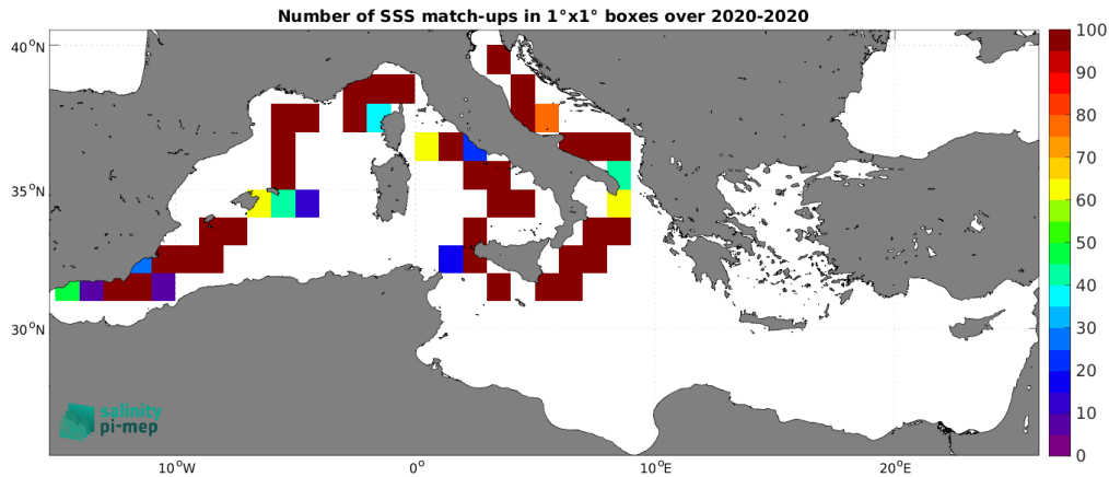
Figure 5: Number of SSS match-ups between Saildrone SSS and the SMOS SSS L3 v332 - 9 Days (CATDS-CPDC) SSS product for the Mediterranean Sea Pi-MEP region over 1^\circ \times 1^\circ boxes and for the full satellite product period.
