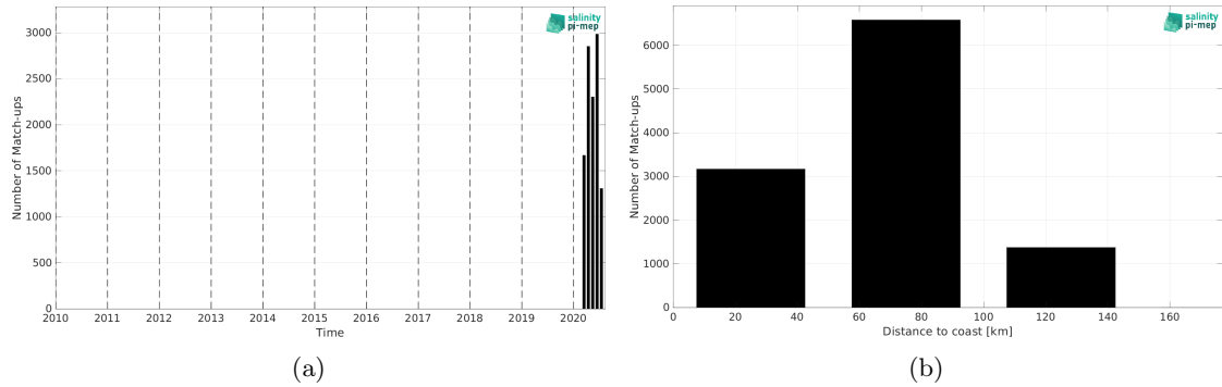
Figure 2: Number of match-ups between Saildrone and SMOS SSS L3 v332 - 9 Days (CATDS-CPDC) SSS as a function of time (a) and as function of the distance to coast (b) over the Mediterranean Sea Pi-MEP region and for the full satellite product period.
