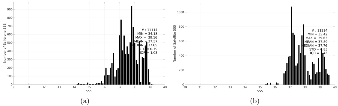
Figure 3: Histograms of SSS from Saildrone (a) and SMOS SSS L3 v332 - 9 Days (CATDS-CPDC) (b) considering all match-up pairs per bins of 0.1 over the Mediterranean Sea Pi-MEP region and for the full satellite product period.
