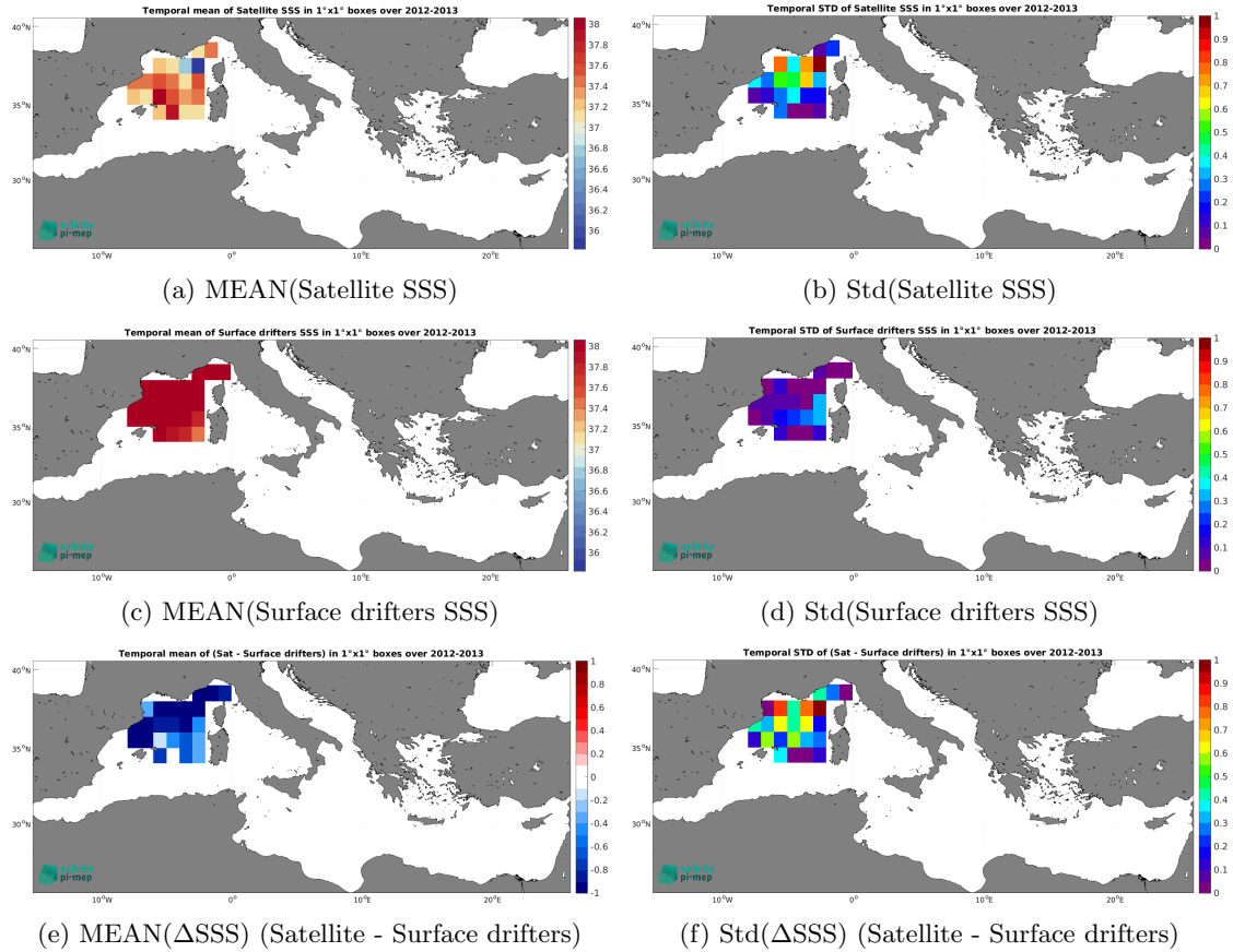
Figure 6: Temporal mean (left) and Std (right) of SSS from SMOS SSS L3 v332 - 9 Days (CATDS-CPDC) (top), Surface drifters (middle), and of \Delta SSS (Satellite - Surface drifters). Only match-up pairs are used to generate these maps.
