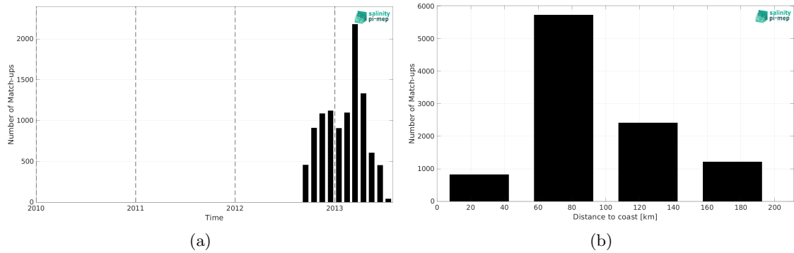
Figure 2: Number of match-ups between Surface drifters and SMOS SSS L3 v332 - 9 Days (CATDS-CPDC) SSS as a function of time (a) and as function of the distance to coast (b) over the Mediterranean Sea Pi-MEP region and for the full satellite product period.
