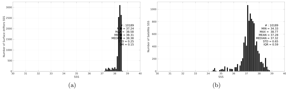
Figure 3: Histograms of SSS from Surface drifters (a) and SMOS SSS L3 v332 - 9 Days (CATDS-CPDC) (b) considering all match-up pairs per bins of 0.1 over the Mediterranean Sea Pi-MEP region and for the full satellite product period.
