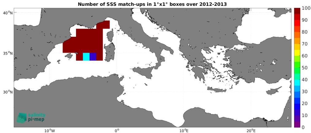
Figure 4: Number of SSS match-ups between Surface drifters SSS and the SMOS SSS L3 v332 - 9 Days (CATDS-CPDC) SSS product for the Mediterranean Sea Pi-MEP region over 1^\circ \times 1^\circ boxes and for the full satellite product period.
