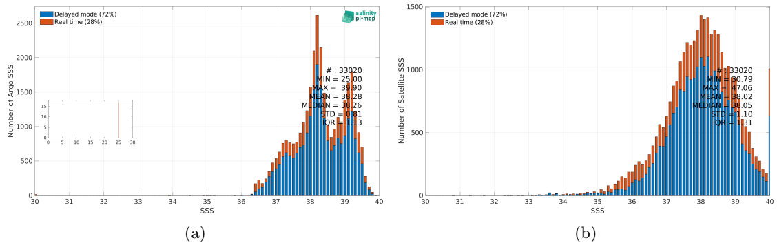
Figure 3: Histograms of SSS from Argo (a) and SMOS SSS L3 v332 - 9 Days (CATDS-CPDC) (b) considering all match-up pairs per bins of 0.1 over the Mediterranean Sea Pi-MEP region and for the full satellite product period.
