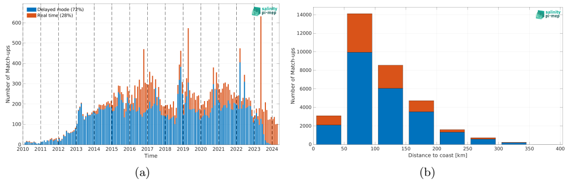
Figure 2: Number of match-ups between Argo and SMOS SSS L3 v332 - 9 Days (CATDS-CPDC) SSS as a function of time (a) and as function of the distance to coast (b) over the Mediterranean Sea Pi-MEP region and for the full satellite product period.
