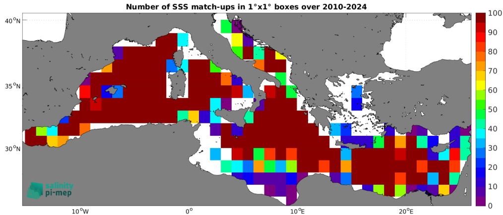
Figure 5: Number of SSS match-ups between Argo SSS and the SMOS SSS L3 v332 - 9 Days (CATDS-CPDC) SSS product for the Mediterranean Sea Pi-MEP region over 1^\circ \times 1^\circ boxes and for the full satellite product period.
