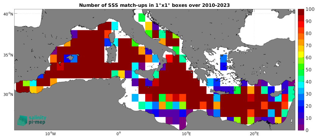
Figure 4: Number of SSS match-ups between Argo SSS and the SMOS SSS L3 v332 - 9 Days (CATDS-CPDC) SSS product for the Mediterranean Sea Pi-MEP region over 1^\circ \times 1^\circ boxes and for the full satellite product period.
