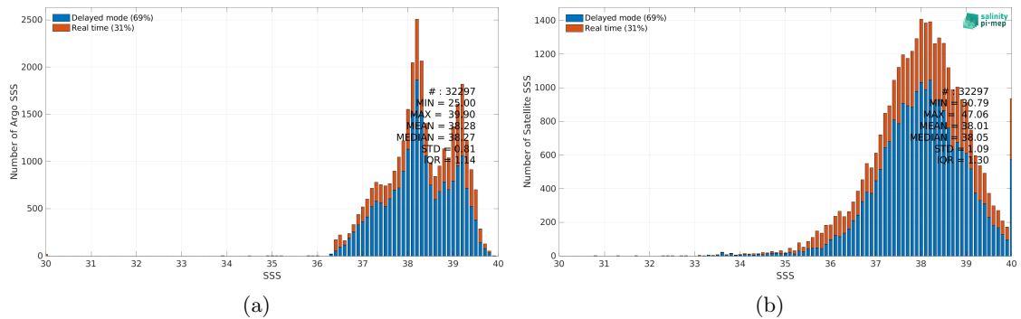
Figure 2: Histograms of SSS from Argo (a) and SMOS SSS L3 v332 - 9 Days (CATDS-CPDC) (b) considering all match-up pairs per bins of 0.1 over the Mediterranean Sea Pi-MEP region and for the full satellite product period.
