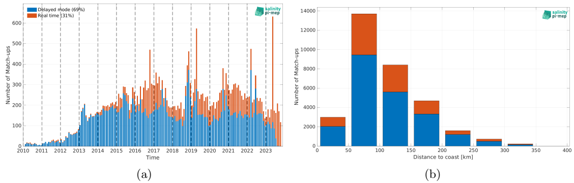
Figure 1: Number of match-ups between Argo and SMOS SSS L3 v332 - 9 Days (CATDS-CPDC) SSS as a function of time (a) and as function of the distance to coast (b) over the Mediterranean Sea Pi-MEP region and for the full satellite product period.
