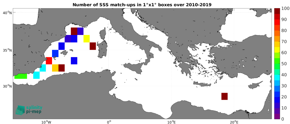
Figure 4: Number of SSS match-ups between TSG (GOSUD-Research-vessel) SSS and the SMOS SSS L2Q v331 - 0.25 Deg (CATDS-CPDC) SSS product for the Mediterranean Sea Pi-MEP region over 1^\circ \times 1^\circ boxes and for the full satellite product period.
