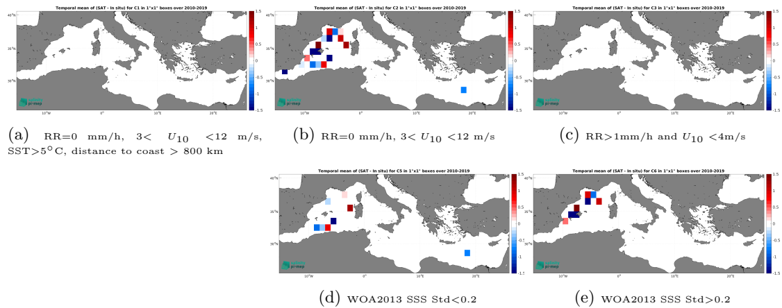
Figure 12: Temporal mean gridded over spatial boxes of size 1^{\circ}\times 1^{\circ} of \Delta SSS (SMOS SSS L2Q v331 - 0.25 Deg (CATDS-CPDC) - TSG (GOSUD-Research-vessel)) for 5 different subdatasets corresponding to:RR=0 mm/h, 3 < U_{10} < 12 m/s, SST >5^{\circ}\text{C} , distance to coast > 800 km (a), RR=0 mm/h, 3 < U_{10} < 12 m/s (b), RR >1 mm/h and U_{10} < 4 m/s (c), WOA2013 SSS Std <0.2 (d), WOA2013 SSS Std >0.2 (e).
