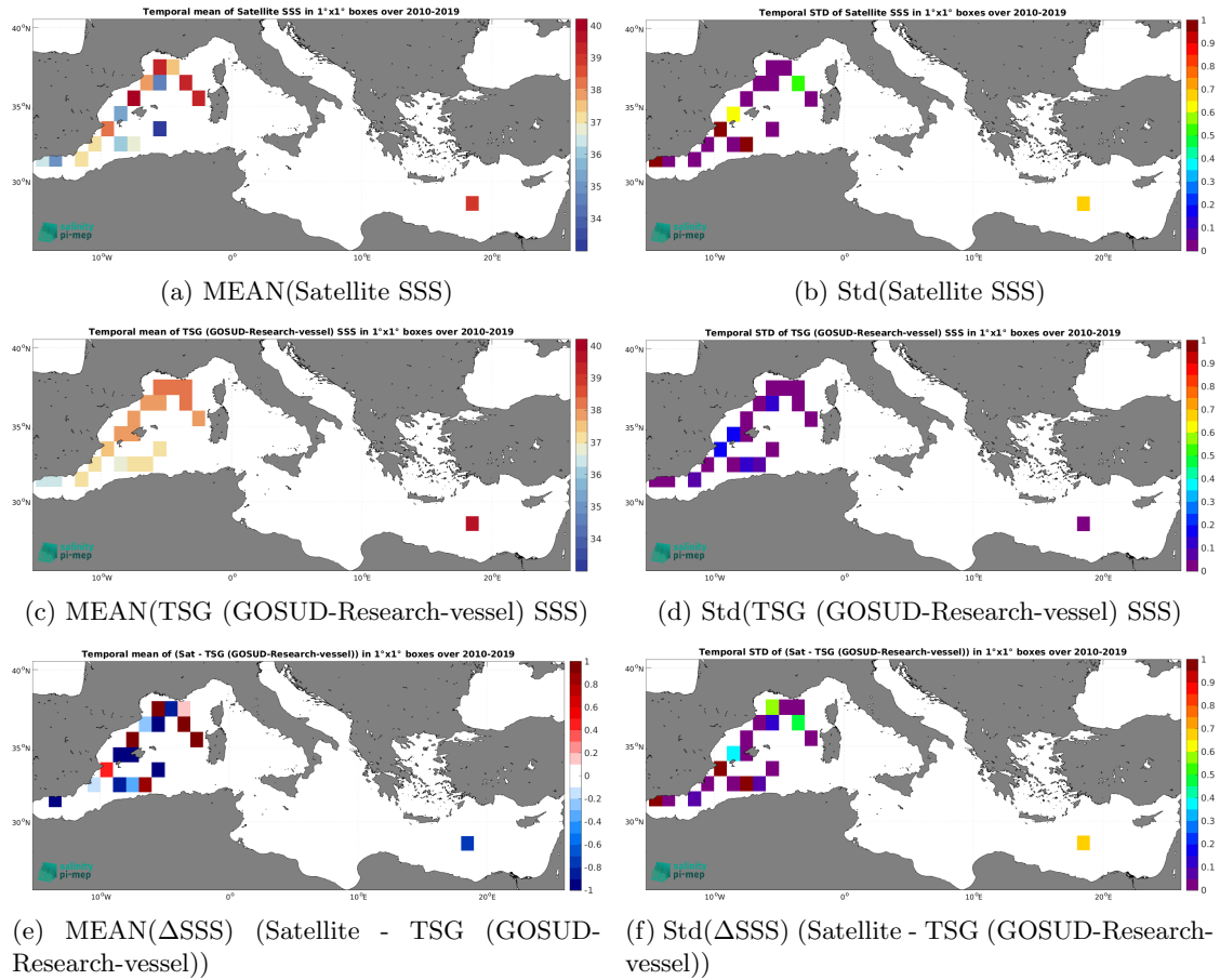
Figure 6: Temporal mean (left) and Std (right) of SSS from SMOS SSS L2Q v331 - 0.25 Deg (CATDS-CPDC) (top), TSG (GOSUD-Research-vessel) (middle), and of \Delta SSS (Satellite - TSG (GOSUD-Research-vessel)). Only match-up pairs are used to generate these maps.
