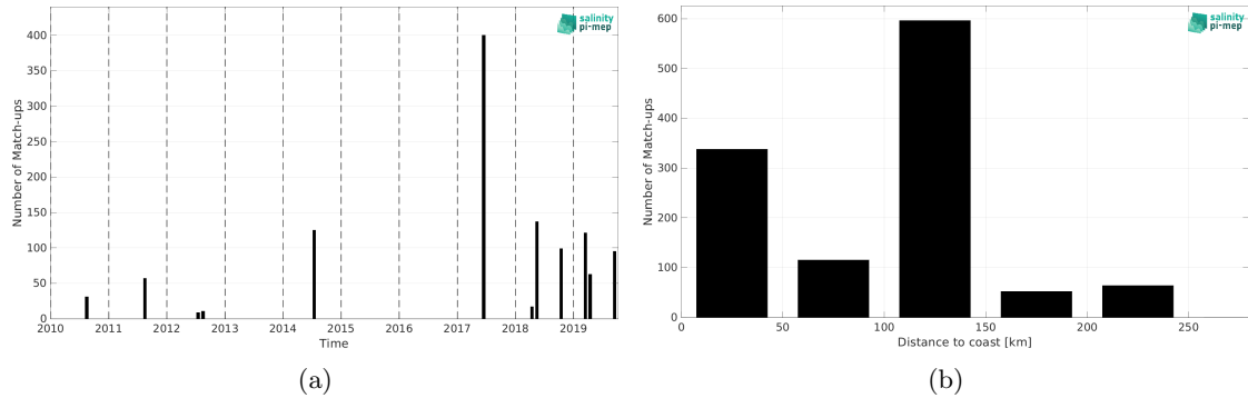
Figure 1: Number of match-ups between TSG (GOSUD-Research-vessel) and SMOS SSS L2Q v331 - 0.25 Deg (CATDS-CPDC) SSS as a function of time (a) and as function of the distance to coast (b) over the Mediterranean Sea Pi-MEP region and for the full satellite product period.
