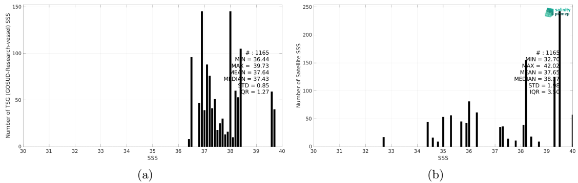
Figure 2: Histograms of SSS from TSG (GOSUD-Research-vessel) (a) and SMOS SSS L2Q v331 - 0.25 Deg (CATDS-CPDC) (b) considering all match-up pairs per bins of 0.1 over the Mediterranean Sea Pi-MEP region and for the full satellite product period.
