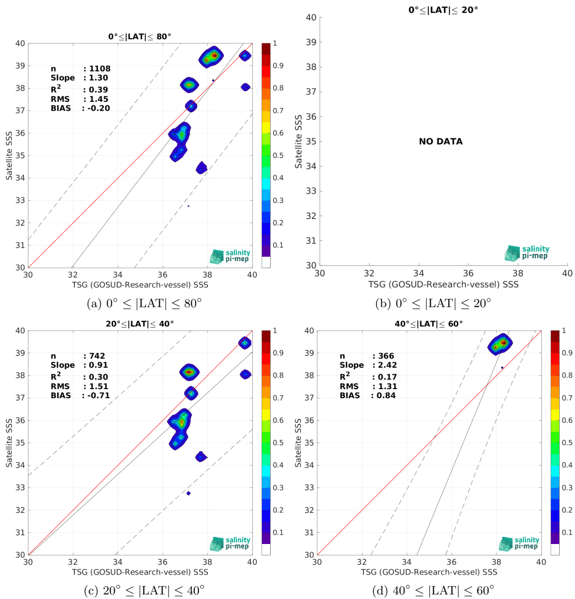
Figure 9: Contour maps of the concentration of SMOS SSS L2Q v331 - 0.25 Deg (CATDS-CPDC) SSS (y-axis) versus TSG (GOSUD-Research-vessel) SSS (x-axis) at match-up pairs for different latitude bands. For each plot, the red line shows x=y . The black thin and dashed lines indicate a linear fit through the data cloud and the \pm 95\% confidence levels, respectively. The number match-up pairs n , the slope and R^2 coefficient of the linear fit, the root mean square (RMS) and the mean bias between satellite and in situ data are indicated for each latitude band in each plots.
