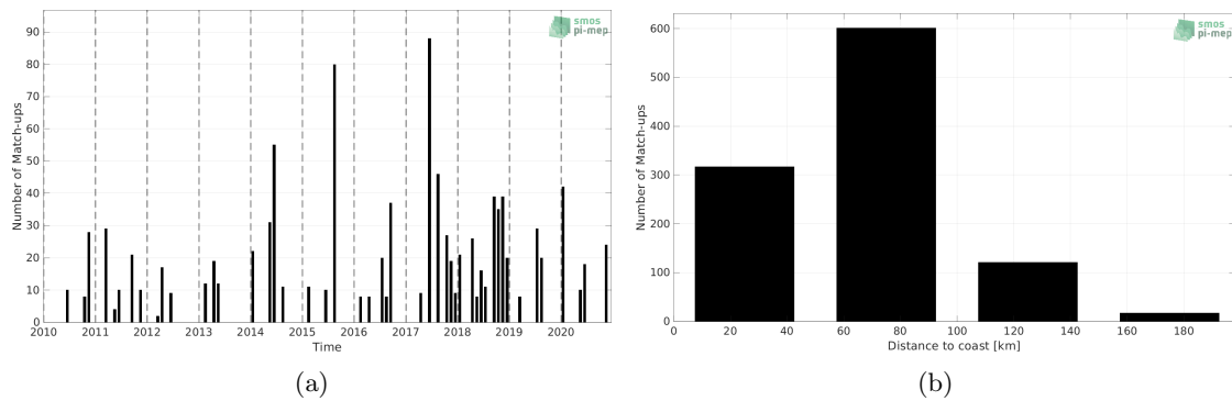
Figure 1: Number of match-ups between TSG (LEGOS-DM) and SMOS SSS L2Q v330 - 0.25 Deg (CATDS-CPDC) SSS as a function of time (a) and as function of the distance to coast (b) over the Mediterranean Sea Pi-MEP region and for the full satellite product period.
