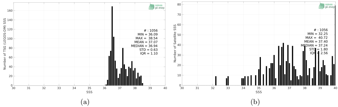
Figure 2: Histograms of SSS from TSG (LEGOS-DM) (a) and SMOS SSS L2Q v330 - 0.25 Deg (CATDS-CPDC) (b) considering all match-up pairs per bins of 0.1 over the Mediterranean Sea Pi-MEP region and for the full satellite product period.
