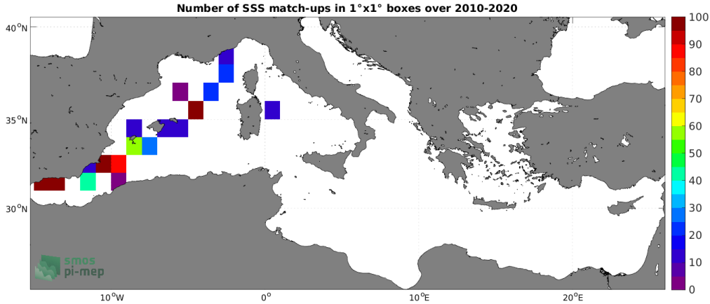
Figure 4: Number of SSS match-ups between TSG (LEGOS-DM) SSS and the SMOS SSS L2Q v330 - 0.25 Deg (CATDS-CPDC) SSS product for the Mediterranean Sea Pi-MEP region over 1^\circ \times 1^\circ boxes and for the full satellite product period.
