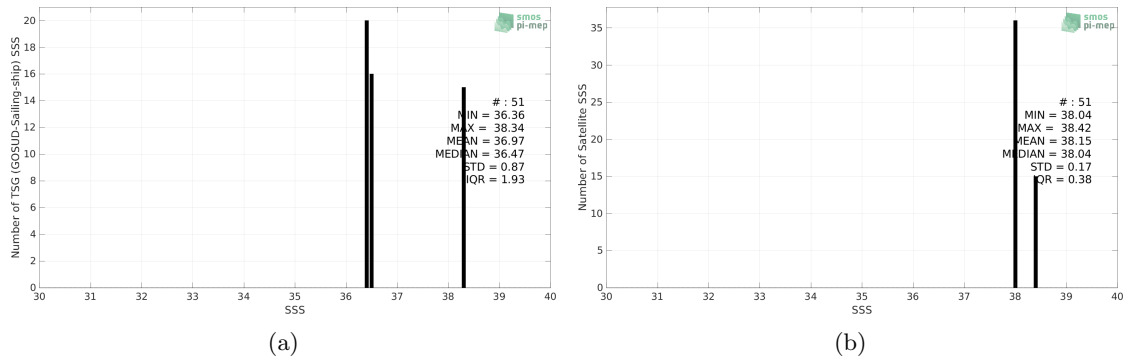
Figure 2: Histograms of SSS from TSG (GOSUD-Sailing-ship) (a) and SMOS SSS L2Q v330 - 0.25 Deg (CATDS-CPDC) (b) considering all match-up pairs per bins of 0.1 over the Mediterranean Sea Pi-MEP region and for the full satellite product period.
