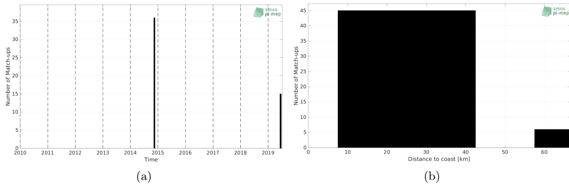
Figure 1: Number of match-ups between TSG (GOSUD-Sailing-ship) and SMOS SSS L2Q v330 - 0.25 Deg (CATDS-CPDC) SSS as a function of time (a) and as function of the distance to coast (b) over the Mediterranean Sea Pi-MEP region and for the full satellite product period.
