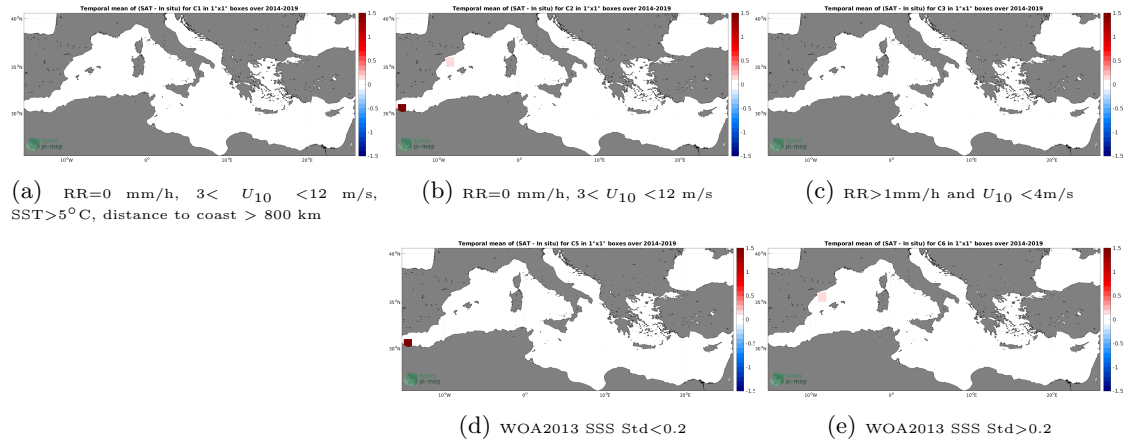
Figure 12: Temporal mean gridded over spatial boxes of size 1^{\circ}\times 1^{\circ} of \Delta SSS (SMOS SSS L2Q v330 - 0.25 Deg (CATDS-CPDC) - TSG (GOSUD-Sailing-ship)) for 5 different subdatasets corresponding to:RR=0 mm/h, 3 < U_{10} < 12 m/s, SST >5^{\circ}\text{C} , distance to coast > 800 km (a), RR=0 mm/h, 3 < U_{10} < 12 m/s (b), RR >1 mm/h and U_{10} < 4 m/s (c), WOA2013 SSS Std <0.2 (d), WOA2013 SSS Std >0.2 (e).
