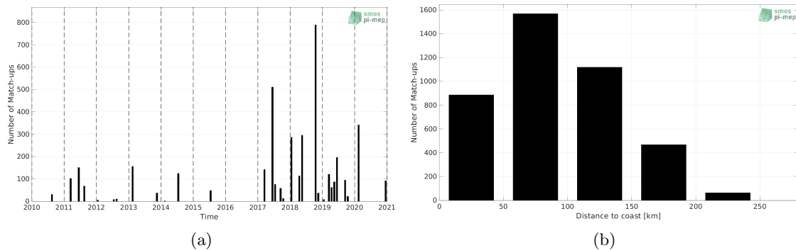
Figure 1: Number of match-ups between TSG (GOSUD-Research-vessel) and SMOS SSS L2Q v330 - 0.25 Deg (CATDS-CPDC) SSS as a function of time (a) and as function of the distance to coast (b) over the Mediterranean Sea Pi-MEP region and for the full satellite product period.
