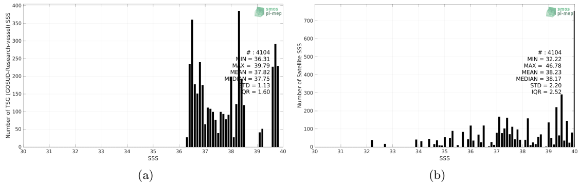
Figure 2: Histograms of SSS from TSG (GOSUD-Research-vessel) (a) and SMOS SSS L2Q v330 - 0.25 Deg (CATDS-CPDC) (b) considering all match-up pairs per bins of 0.1 over the Mediterranean Sea Pi-MEP region and for the full satellite product period.
