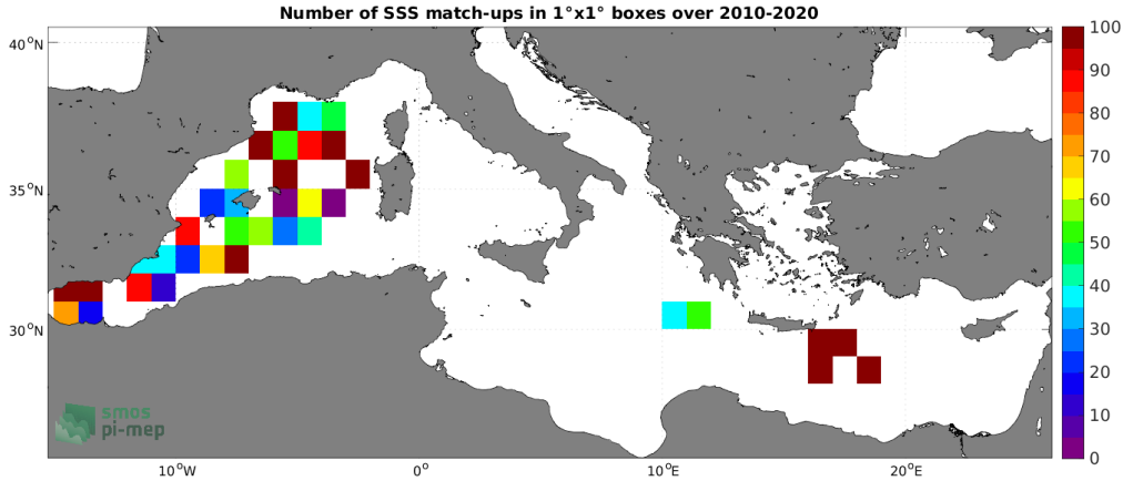
Figure 4: Number of SSS match-ups between TSG (GOSUD-Research-vessel) SSS and the SMOS SSS L2Q v330 - 0.25 Deg (CATDS-CPDC) SSS product for the Mediterranean Sea Pi-MEP region over 1^\circ \times 1^\circ boxes and for the full satellite product period.
