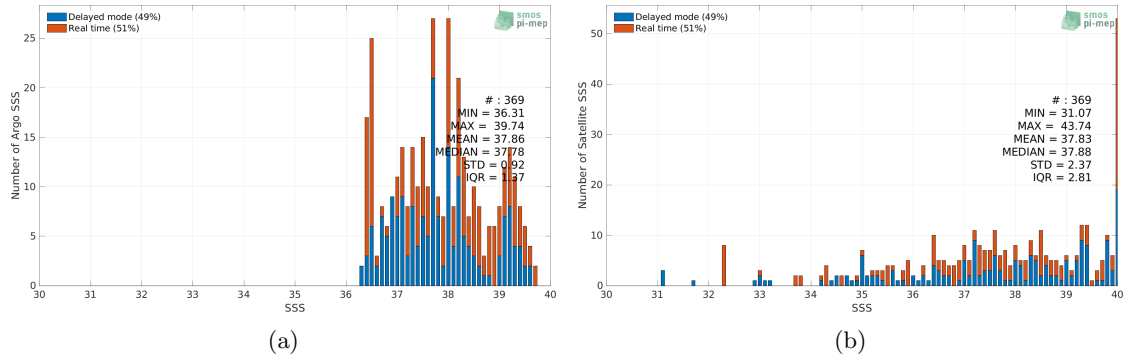
Figure 2: Histograms of SSS from Argo (a) and SMOS SSS L2Q v330 - 0.25 Deg (CATDS-CPDC) (b) considering all match-up pairs per bins of 0.1 over the Mediterranean Sea Pi-MEP region and for the full satellite product period.
