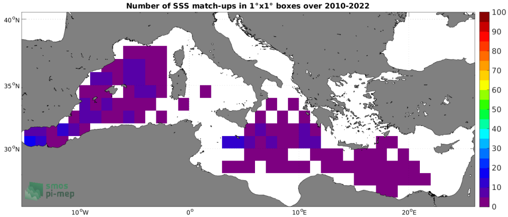
Figure 4: Number of SSS match-ups between Argo SSS and the SMOS SSS L2Q v330 - 0.25 Deg (CATDS-CPDC) SSS product for the Mediterranean Sea Pi-MEP region over 1^\circ \times 1^\circ boxes and for the full satellite product period.
