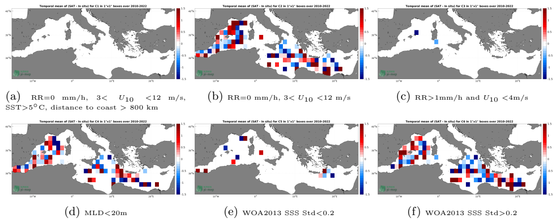
Figure 12: Temporal mean gridded over spatial boxes of size 1^\circ \times 1^\circ of \Delta SSS (SMOS SSS L2Q v330 - 0.25 Deg (CATDS-CPDC) - Argo) for 6 different subdatasets corresponding to:RR=0 mm/h, 3 < U_{10} < 12 m/s, SST >5^\circ C, distance to coast > 800 km (a), RR=0 mm/h, 3 < U_{10} < 12 m/s (b), RR >1 mm/h and U_{10} < 4 m/s (c),MLD <20 m (d),WOA2013 SSS Std <0.2 (e),WOA2013 SSS Std >0.2 (f).
