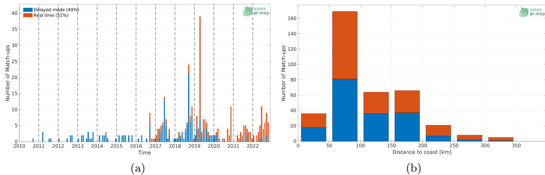
Figure 1: Number of match-ups between Argo and SMOS SSS L2Q v330 - 0.25 Deg (CATDS-CPDC) SSS as a function of time (a) and as function of the distance to coast (b) over the Mediterranean Sea Pi-MEP region and for the full satellite product period.
