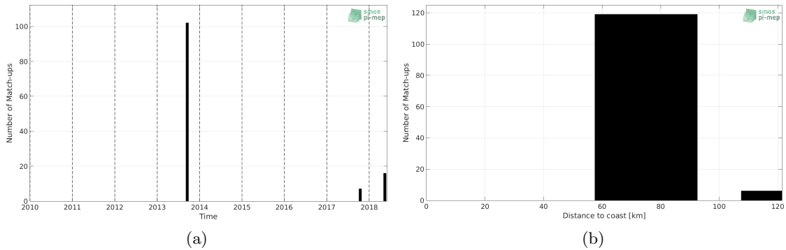
Figure 1: Number of match-ups between TSG-GOSUD-Research-vessel and SMOS-L3-CATDS-CPDC-V321-L2Q SSS as a function of time (a) and as function of the distance to coast (b) over the Mediterranean Sea Pi-MEP region and for the full satellite product period.
