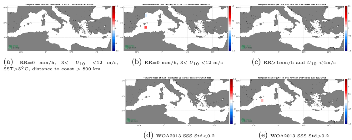
Figure 12: Temporal mean gridded over spatial boxes of size 1^\circ \times 1^\circ of \Delta SSS (SMOS-L3-CATDS-CPDC-V321-L2Q - TSG-GOSUD-Research-vessel) for 5 different subdatasets corresponding to:RR=0 mm/h, 3 < U_{10} < 12 m/s, SST>5°C, distance to coast > 800 km (a), RR=0 mm/h, 3 < U_{10} < 12 m/s (b), RR>1mm/h and U_{10} < 4 m/s (c), WOA2013 SSS Std<0.2 (d), WOA2013 SSS Std>0.2 (e).
