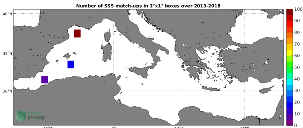
Figure 4: Number of SSS match-ups between TSG-GOSUD-Research-vessel SSS and the SMOS-L3-CATDS-CPDC-V321-L2Q SSS product for the Mediterranean Sea Pi-MEP region over 1°x1° boxes and for the full satellite product period.
