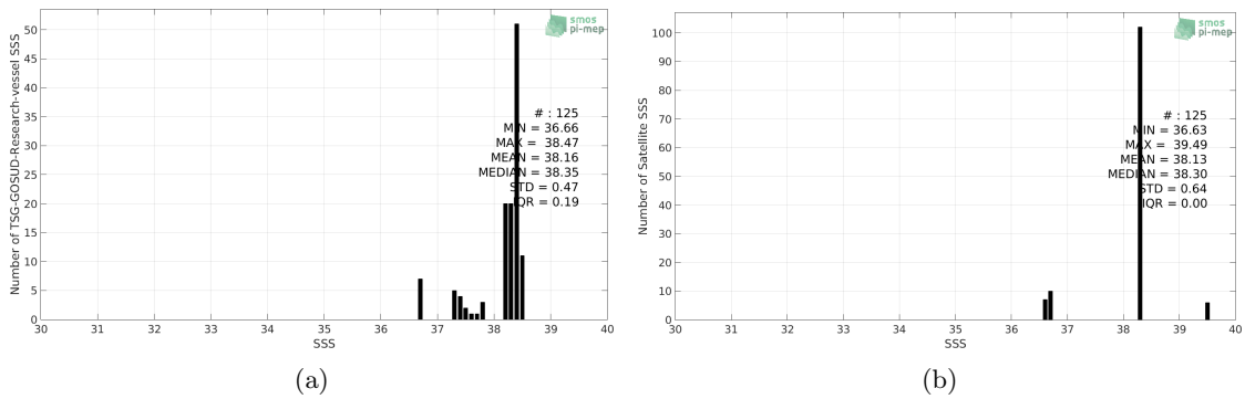
Figure 2: Histograms of SSS from TSG-GOSUD-Research-vessel (a) and SMOS-L3-CATDS-CPDC-V321-L2Q (b) considering all match-up pairs per bins of 0.1 over the Mediterranean Sea Pi-MEP region and for the full satellite product period.
