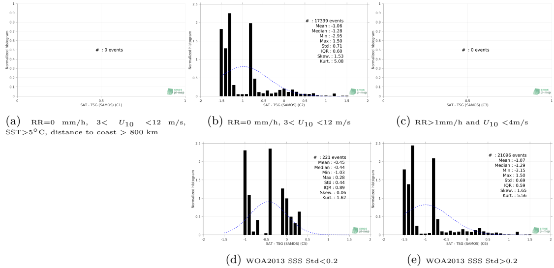
Figure 13: Normalized histogram of \Delta\text{SSS} (SMOS SSS L3 v317 - Monthly - 25 km (CATDS-CPDC) - TSG (SAMOS)) for 5 different subdatasets corresponding to: RR=0 mm/h, 3 < U_{10} < 12 m/s, SST > 5^\circ\text{C} , distance to coast > 800 km (a), RR=0 mm/h, 3 < U_{10} < 12 m/s (b), RR > 1\text{mm/h} and U_{10} < 4\text{m/s} (c), WOA2013 SSS Std < 0.2 (d), WOA2013 SSS Std > 0.2 (e).
