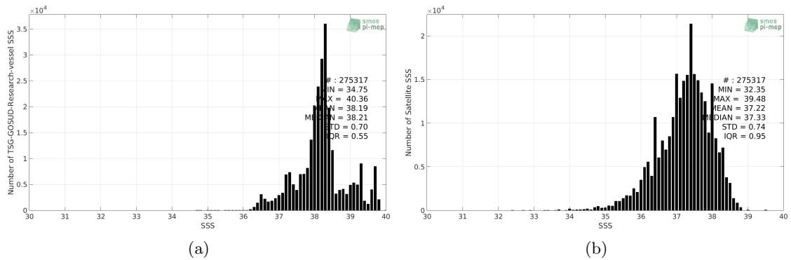
Figure 2: Histograms of SSS from TSG-GOSUD-Research-vessel (a) and SMOS L3 v317 - Monthly - 25 km (CATDS-CPDC) (b) considering all match-up pairs per bins of 0.1 over the Mediterranean Sea Pi-MEP region and for the full satellite product period.
