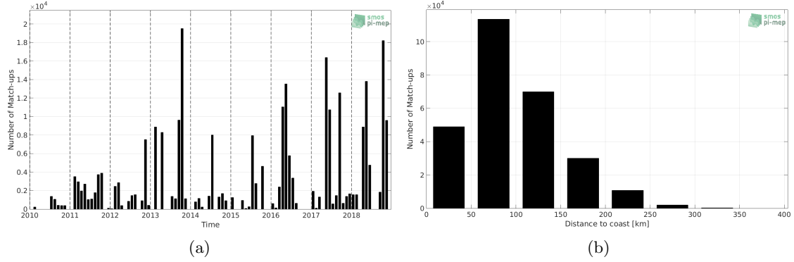
Figure 1: Number of match-ups between TSG-GOSUD-Research-vessel and SMOS L3 v317 - Monthly - 25 km (CATDS-CPDC) SSS as a function of time (a) and as function of the distance to coast (b) over the Mediterranean Sea Pi-MEP region and for the full satellite product period.
