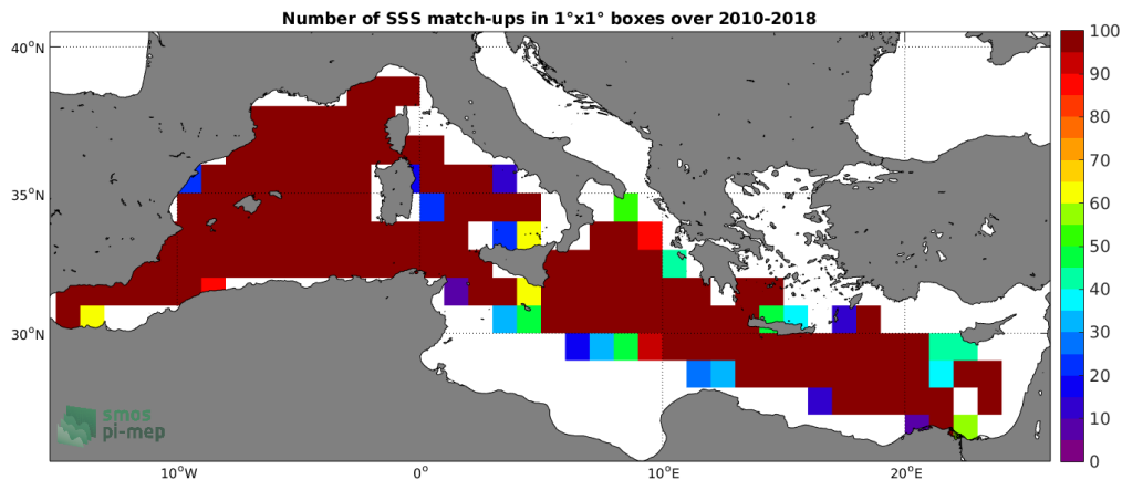
Figure 4: Number of SSS match-ups between TSG-GOSUD-Research-vessel SSS and the SMOS L3 v317 - Monthly - 25 km (CATDS-CPDC) SSS product for the Mediterranean Sea Pi-MEP region over 1^\circ \times 1^\circ boxes and for the full satellite product period.
