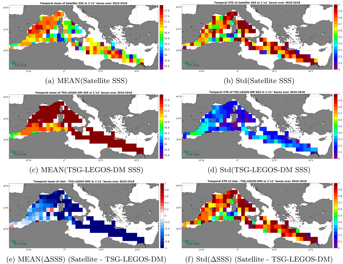
Figure 6: Temporal mean (left) and Std (right) of SSS from SMOS L3 v317 - 10 Days - 25 km (CATDS-CPDC) (top), TSG-LEGOS-DM (middle), and of \Delta SSS (Satellite - TSG-LEGOS-DM). Only match-up pairs are used to generate these maps.
