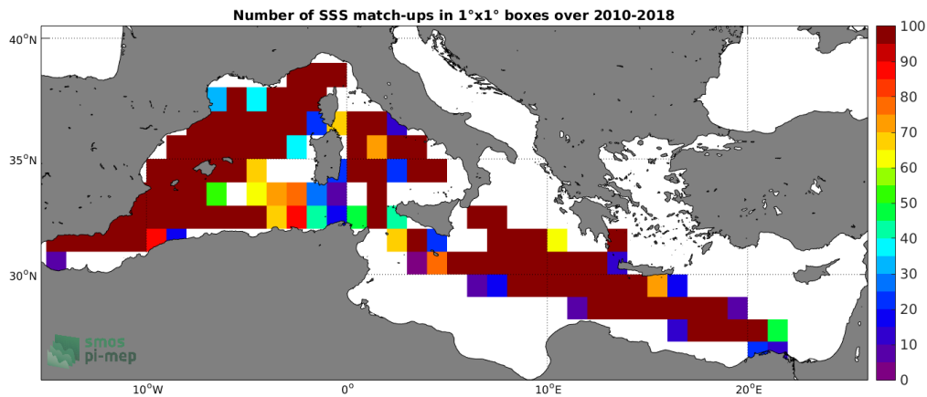
Figure 4: Number of SSS match-ups between TSG-LEGOS-DM SSS and the SMOS L3 v317 - 10 Days - 25 km (CATDS-CPDC) SSS product for the Mediterranean Sea Pi-MEP region over 1^\circ \times 1^\circ boxes and for the full satellite product period.
