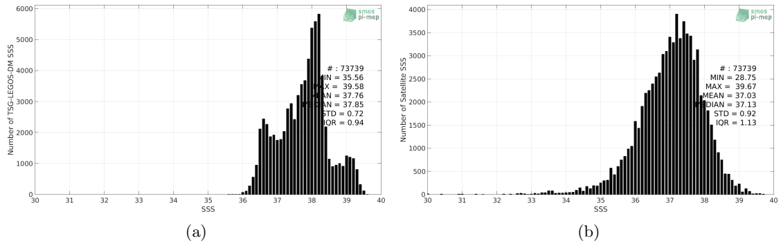
Figure 2: Histograms of SSS from TSG-LEGOS-DM (a) and SMOS L3 v317 - 10 Days - 25 km (CATDS-CPDC) (b) considering all match-up pairs per bins of 0.1 over the Mediterranean Sea Pi-MEP region and for the full satellite product period.
