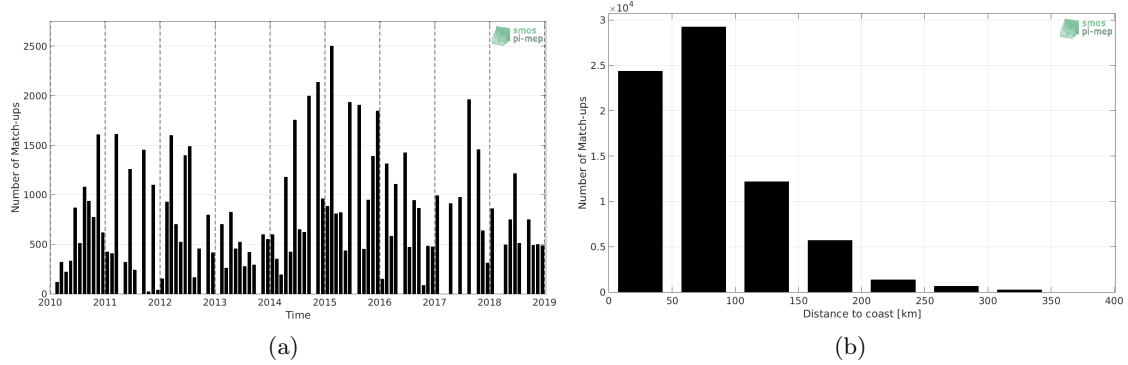
Figure 1: Number of match-ups between TSG-LEGOS-DM and SMOS L3 v317 - 10 Days - 25 km (CATDS-CPDC) SSS as a function of time (a) and as function of the distance to coast (b) over the Mediterranean Sea Pi-MEP region and for the full satellite product period.
