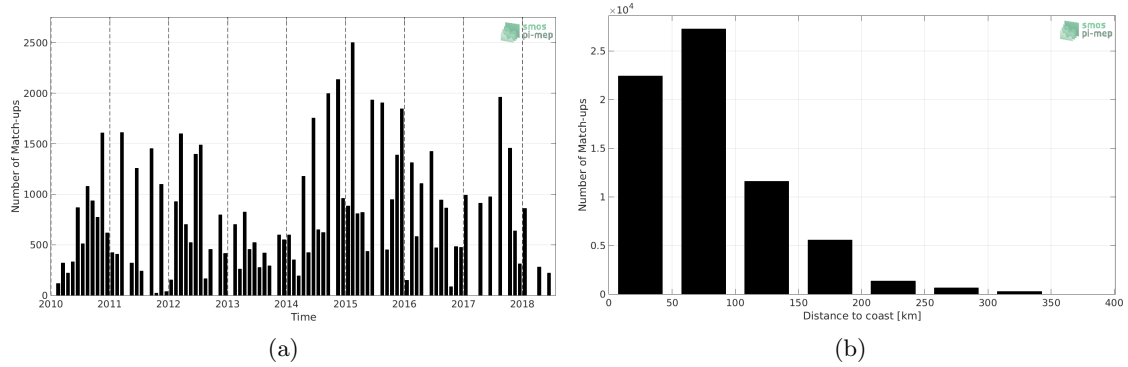
Figure 1: Number of match-ups between TSG-LEGOS-DM and SMOS-L3-CATDS-CPDC-V317-10DAYS-25KM SSS as a function of time (a) and as function of the distance to coast (b) over the Mediterranean Sea Pi-MEP region and for the full satellite product period.
