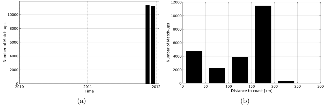
Figure 1: Number of match-ups between TSG-SAMOS and SMOS-L3-CATDS-CPDC-V3-MONTHLY-25KM SSS as a function of time (a) and as function of the distance to coast (b) over the Mediterranean Sea Pi-MEP region and for the full satellite product period.
