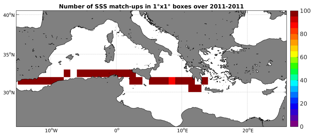
Figure 4: Number of SSS match-ups between TSG-SAMOS SSS and the SMOS-L3-CATDS-CPDC-V3-MONTHLY-25KM SSS product for the Mediterranean Sea Pi-MEP region over 1^\circ \times 1^\circ boxes and for the full satellite product period.
