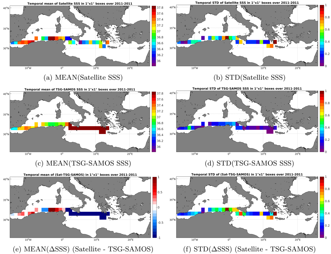
Figure 6: Temporal mean (left) and STD (right) of SSS from SMOS-L3-CATDS-CPDC-V3-MONTHLY-25KM (top), TSG-SAMOS (middle), and of \Delta SSS (Satellite - TSG-SAMOS). Only match-up pairs are used to generate these maps.
