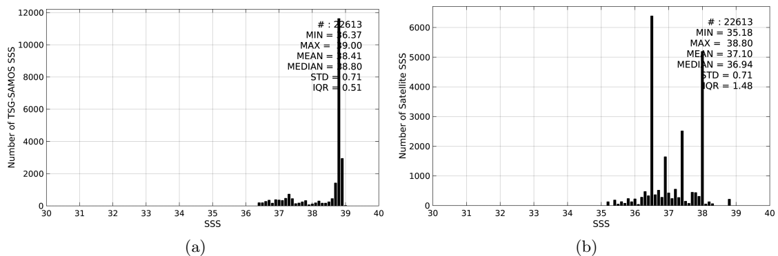
Figure 2: Histograms of SSS from TSG-SAMOS (a) and SMOS-L3-CATDS-CPDC-V3-MONTHLY-25KM (b) considering all match-up pairs per bins of 0.1 over the Mediterranean Sea Pi-MEP region and for the full satellite product period.
