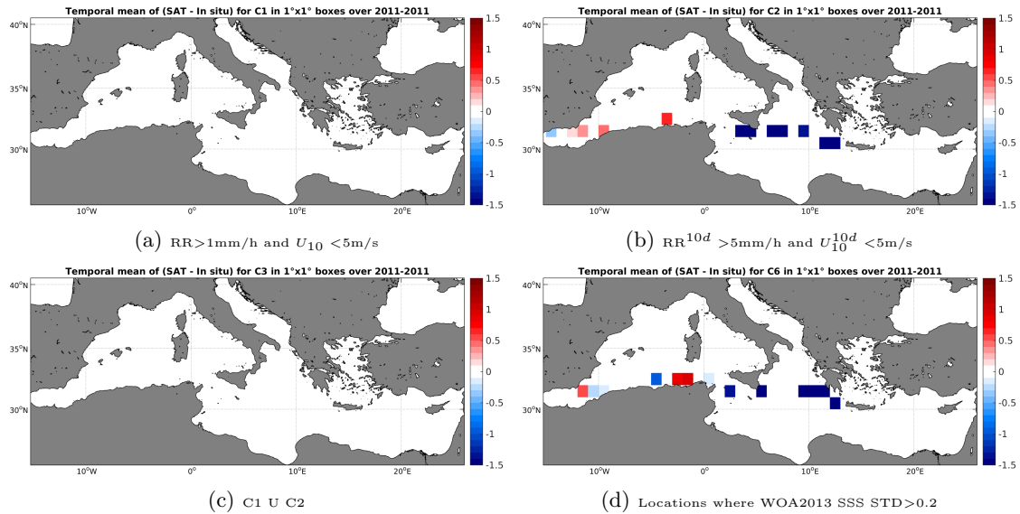
Figure 12: Temporal mean gridded over spatial boxes of size 1^\circ \times 1^\circ of \Delta SSS (SMOS-L3-CATDS-CPDC-V3-MONTHLY-25KM - TSG-SAMOS) for 4 different subdatasets corresponding to:RR > 1 mm/h and U_{10} < 5 m/s (a), RR ^{10d} > 5 mm/h and U_{10}^{10d} < 5 m/s (b), C1 U C2 (c),Locations where WOA2013 SSS STD > 0.2 (d).
