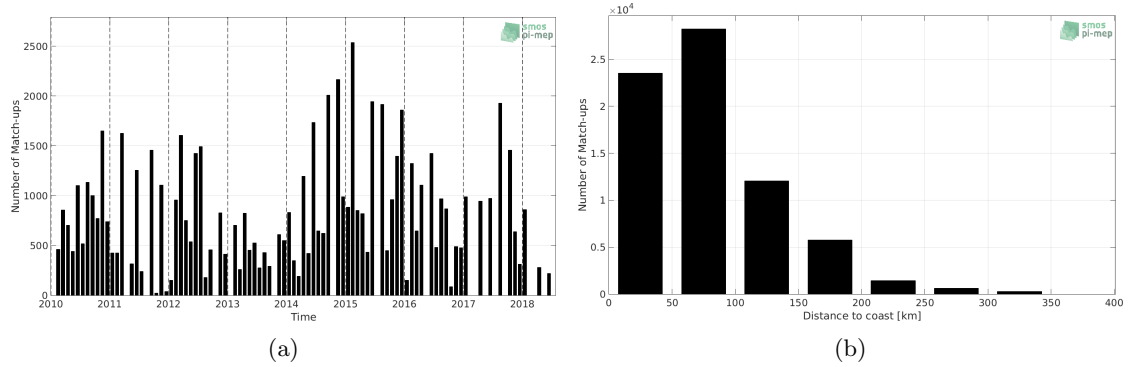
Figure 1: Number of match-ups between TSG-LEGOS-DM and SMOS-L3-CATDS-CPDC-V3-MONTHLY-25KM SSS as a function of time (a) and as function of the distance to coast (b) over the Mediterranean Sea Pi-MEP region and for the full satellite product period.
