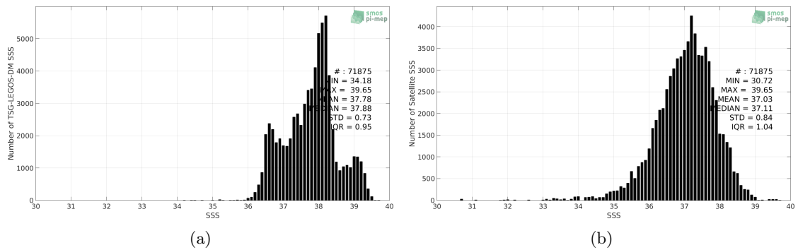
Figure 2: Histograms of SSS from TSG-LEGOS-DM (a) and SMOS-L3-CATDS-CPDC-V3-MONTHLY-25KM (b) considering all match-up pairs per bins of 0.1 over the Mediterranean Sea Pi-MEP region and for the full satellite product period.
