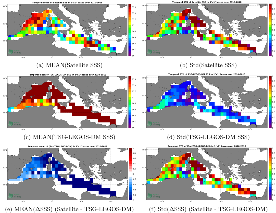
Figure 6: Temporal mean (left) and Std (right) of SSS from SMOS-L3-CATDS-CPDC-V3-MONTHLY-25KM (top), TSG-LEGOS-DM (middle), and of \Delta SSS (Satellite - TSG-LEGOS-DM). Only match-up pairs are used to generate these maps.
