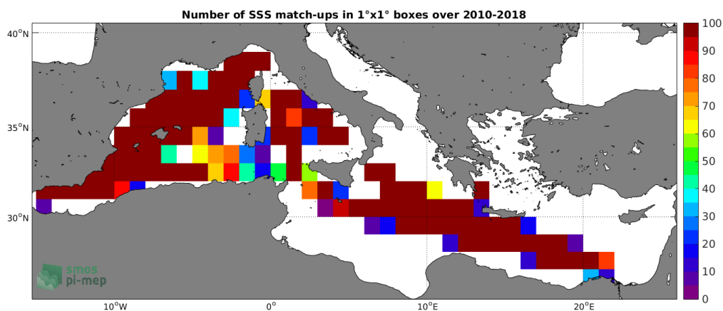
Figure 4: Number of SSS match-ups between TSG-LEGOS-DM SSS and the SMOS-L3-CATDS-CPDC-V3-MONTHLY-25KM SSS product for the Mediterranean Sea Pi-MEP region over 1^\circ \times 1^\circ boxes and for the full satellite product period.
