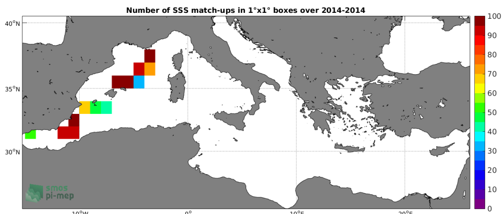
Figure 4: Number of SSS match-ups between TSG-GOSUD-Sailing-ship SSS and the SMOS-L3-CATDS-CPDC-V3-MONTHLY-25KM SSS product for the Mediterranean Sea Pi-MEP region over 1^\circ \times 1^\circ boxes and for the full satellite product period.
