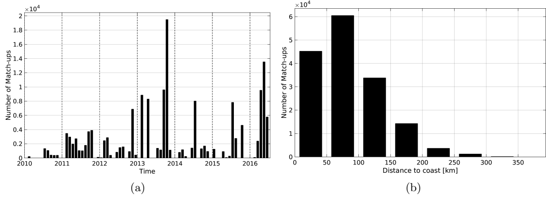
Figure 1: Number of match-ups between TSG-GOSUD-Research-vessel and SMOS-L3-CATDS-CPDC-V3-MONTHLY-25KM SSS as a function of time (a) and as function of the distance to coast (b) over the Mediterranean Sea Pi-MEP region and for the full satellite product period.
