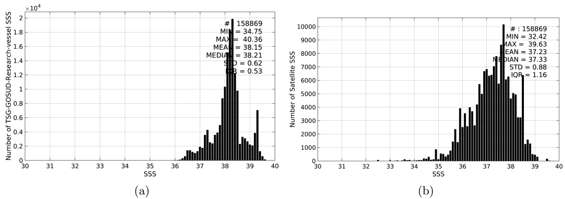
Figure 2: Histograms of SSS from TSG-GOSUD-Research-vessel (a) and SMOS-L3-CATDS-CPDC-V3-MONTHLY-25KM (b) considering all match-up pairs per bins of 0.1 over the Mediterranean Sea Pi-MEP region and for the full satellite product period.
