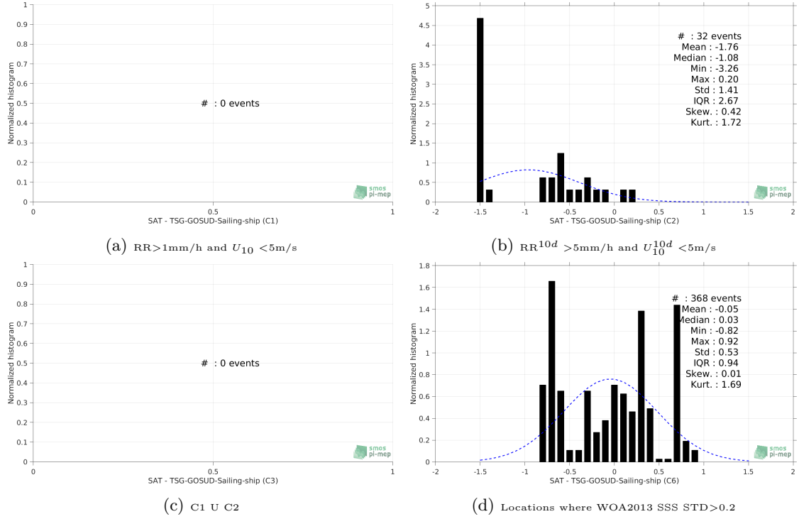
Figure 13: Normalized histogram of \Delta SSS (SMOS-L3-CATDS-CPDC-V3-10DAYS-25KM - TSG-GOSUD-Sailing-ship) for 6 different subdatasets corresponding to: RR > 1\text{mm/h} and U_{10} < 5\text{m/s} (a), RR^{10d} > 5\text{mm/h} and U_{10}^{10d} < 5\text{m/s} (b), C1 \cup C2 (c), Locations where WOA2013 SSS STD > 0.2 (d).
