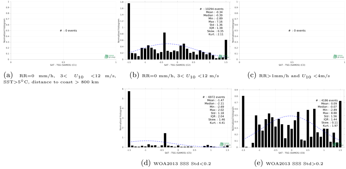
Figure 13: Normalized histogram of \Delta\text{SSS} (SMOS SSS L3 v2 - 9-Days (BEC) - TSG (SAMOS)) for 5 different subdatasets corresponding to: RR=0 mm/h, 3 < U_{10} < 12 m/s, SST>5°C, distance to coast > 800 km (a), RR=0 mm/h, 3 < U_{10} < 12 m/s (b), RR>1mm/h and U_{10} < 4 m/s (c), WOA2013 SSS Std<0.2 (d), WOA2013 SSS Std>0.2 (e).
