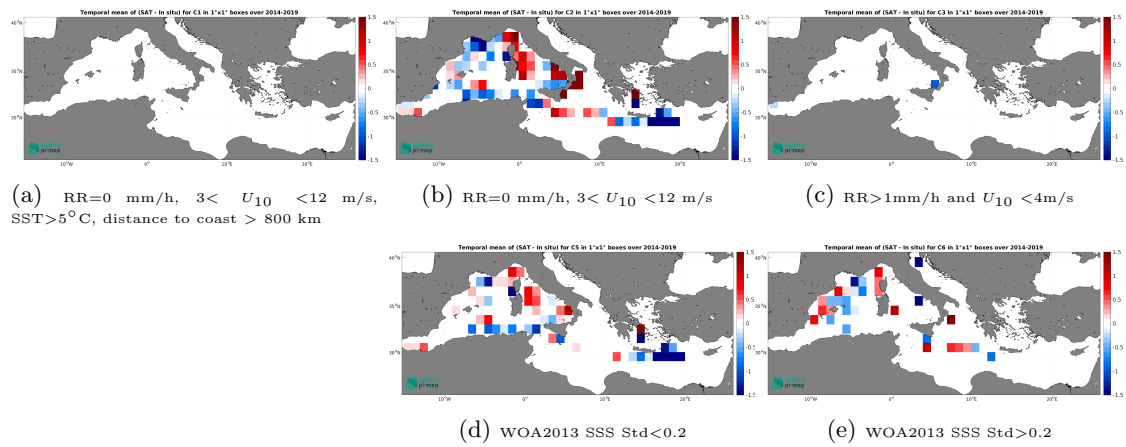
Figure 14: Temporal mean gridded over spatial boxes of size 1^\circ \times 1^\circ of \Delta\text{SSS} (SMOS SSS L3 v2 - 9-Days (BEC) - TSG (GOSUD-Sailing-ship)) for 5 different subdatasets corresponding to:RR=0 mm/h, 3 < U_{10} < 12 m/s, SST >5^\circ\text{C} , distance to coast > 800 km (a), RR=0 mm/h, 3 < U_{10} < 12 m/s (b), RR >1 mm/h and U_{10} < 4 m/s (c), WOA2013 SSS Std <0.2 (d), WOA2013 SSS Std >0.2 (e).
