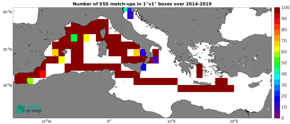
Figure 5: Number of SSS match-ups between TSG (GOSUD-Sailing-ship) SSS and the SMOS SSS L3 v2 - 9-Days (BEC) SSS product for the Mediterranean Sea Pi-MEP region over 1^\circ \times 1^\circ boxes and for the full satellite product period.
