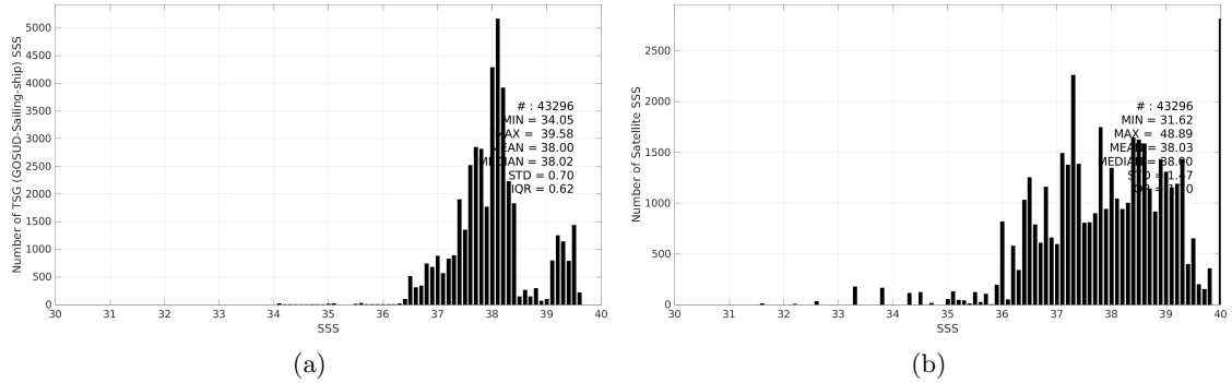
Figure 3: Histograms of SSS from TSG (GOSUD-Sailing-ship) (a) and SMOS SSS L3 v2 - 9-Days (BEC) (b) considering all match-up pairs per bins of 0.1 over the Mediterranean Sea Pi-MEP region and for the full satellite product period.
