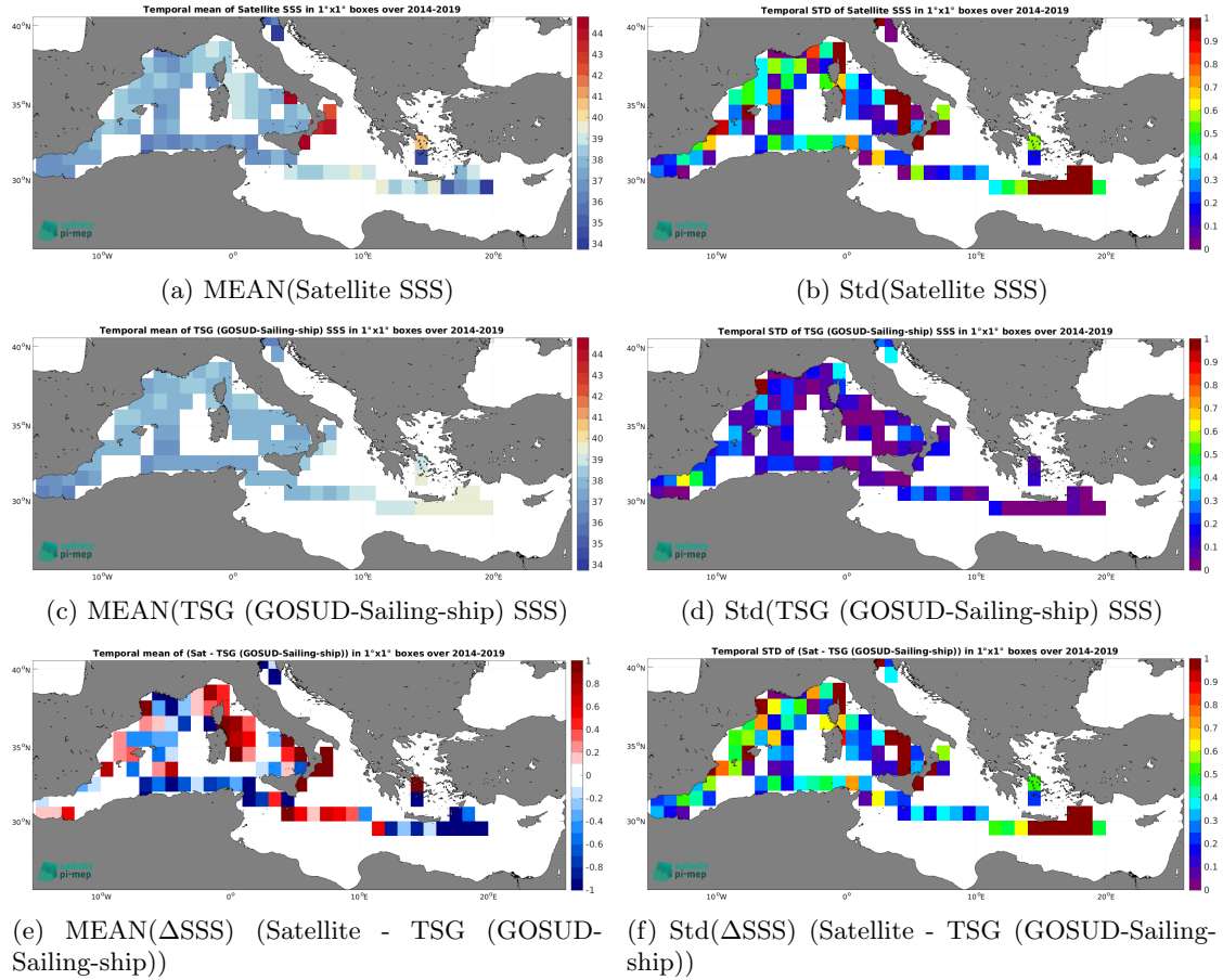
Figure 7: Temporal mean (left) and Std (right) of SSS from SMOS SSS L3 v2 - 9-Days (BEC) (top), TSG (GOSUD-Sailing-ship) (middle), and of \Delta\text{SSS} (Satellite - TSG (GOSUD-Sailing-ship)). Only match-up pairs are used to generate these maps.
