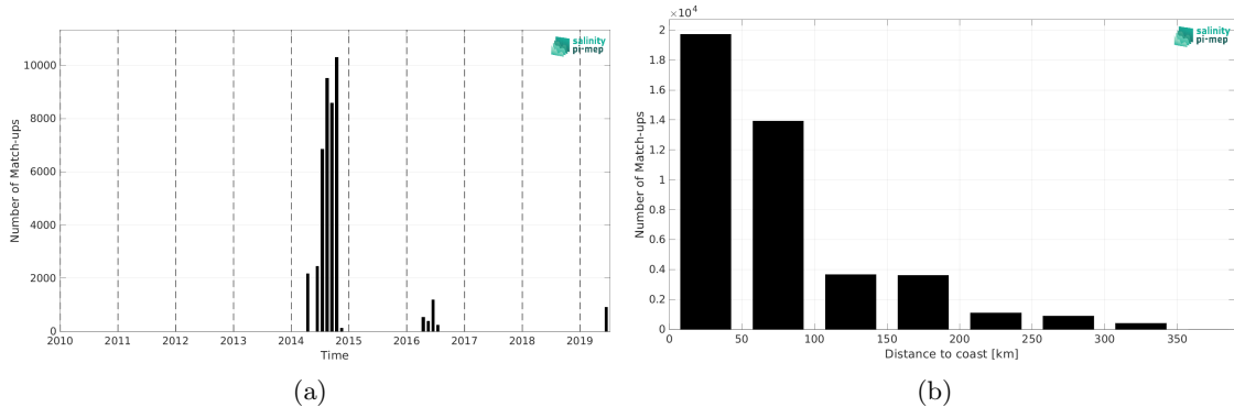
Figure 2: Number of match-ups between TSG (GOSUD-Sailing-ship) and SMOS SSS L3 v2 - 9-Days (BEC) SSS as a function of time (a) and as function of the distance to coast (b) over the Mediterranean Sea Pi-MEP region and for the full satellite product period.
