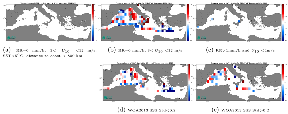
Figure 12: Temporal mean gridded over spatial boxes of size 1^\circ \times 1^\circ of \Delta\text{SSS} (SMOS SSS L3 v2 - 9-Days (BEC) - TSG (GOSUD-Sailing-ship)) for 5 different subdatasets corresponding to:RR=0 mm/h, 3 < U_{10} < 12 m/s, SST>5°C, distance to coast > 800 km (a), RR=0 mm/h, 3 < U_{10} < 12 m/s (b), RR>1mm/h and U_{10} < 4 m/s (c), WOA2013 SSS Std<0.2 (d), WOA2013 SSS Std>0.2 (e).
