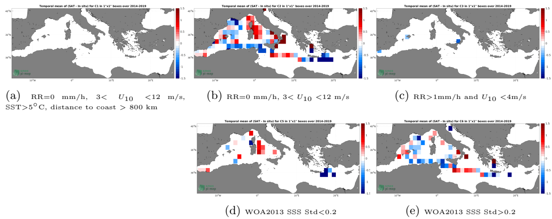
Figure 12: Temporal mean gridded over spatial boxes of size 1^\circ \times 1^\circ of \Delta SSS (SMOS SSS L3 v2 - 9-Days (BEC) - TSG (GOSUD-Sailing-ship)) for 5 different subdatasets corresponding to:RR=0 mm/h, 3 < U_{10} < 12 m/s, SST>5°C, distance to coast > 800 km (a), RR=0 mm/h, 3 < U_{10} < 12 m/s (b), RR>1mm/h and U_{10} < 4 m/s (c), WOA2013 SSS Std<0.2 (d), WOA2013 SSS Std>0.2 (e).
