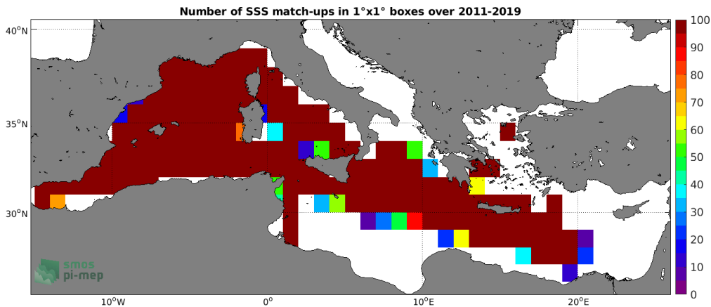
Figure 4: Number of SSS match-ups between TSG (GOSUD-Research-vessel) SSS and the SMOS SSS L3 v2 - 9-Days (BEC) SSS product for the Mediterranean Sea Pi-MEP region over 1°x1° boxes and for the full satellite product period.
