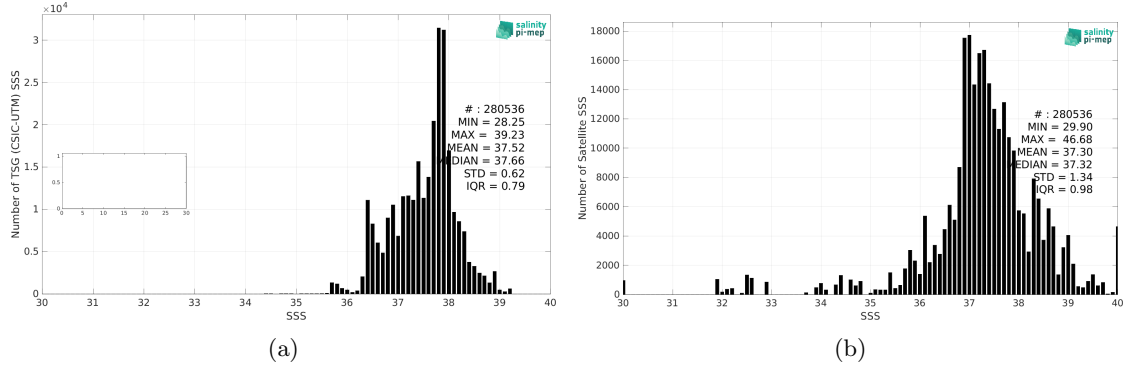
Figure 2: Histograms of SSS from TSG (CSIC-UTM) (a) and SMOS SSS L3 v2 - 9-Days (BEC) (b) considering all match-up pairs per bins of 0.1 over the Mediterranean Sea Pi-MEP region and for the full satellite product period.
