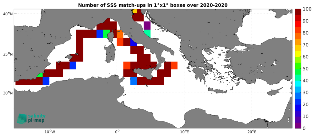
Figure 4: Number of SSS match-ups between Saildrone SSS and the SMOS SSS L3 v2 - 9-Days (BEC) SSS product for the Mediterranean Sea Pi-MEP region over 1^\circ \times 1^\circ boxes and for the full satellite product period.
