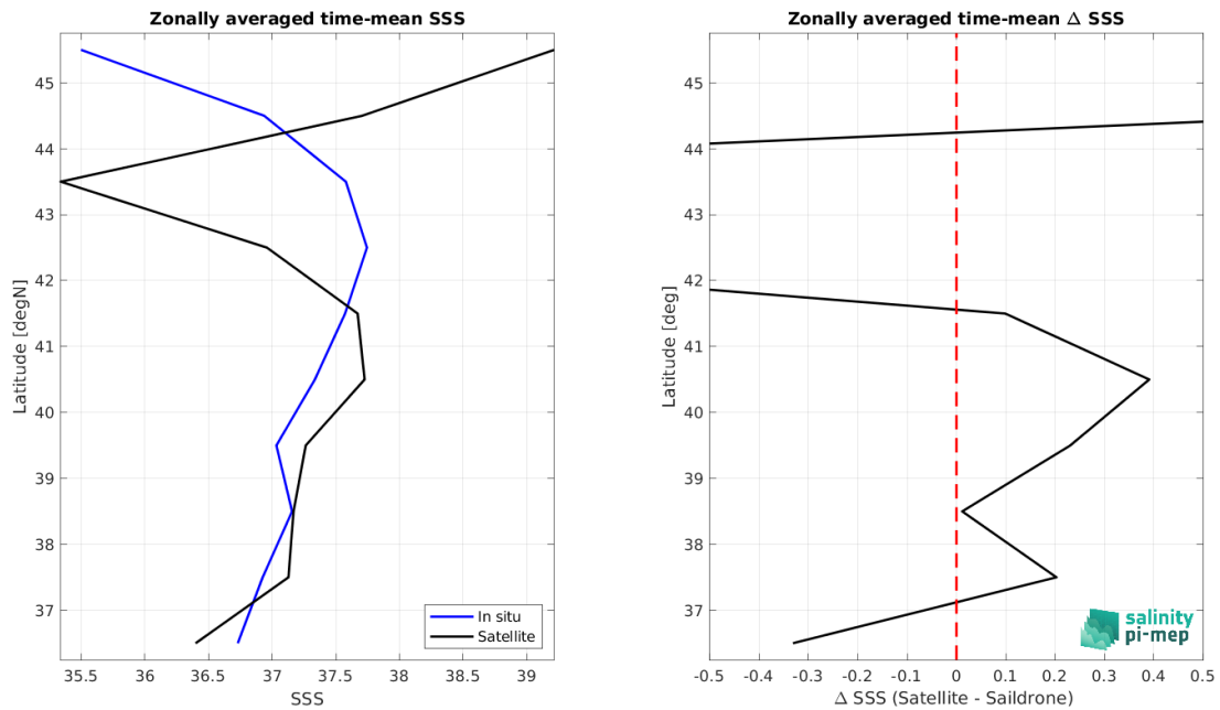
Figure 8: Left panel: Zonal mean SSS from SMOS SSS L3 v2 - 9-Days (BEC) satellite product (black) and from Saildrone (blue). Right panel: Zonal mean of \Delta SSS (Satellite - Saildrone) for all the collected Pi-MEP match-up pairs estimated over the full satellite product period.
