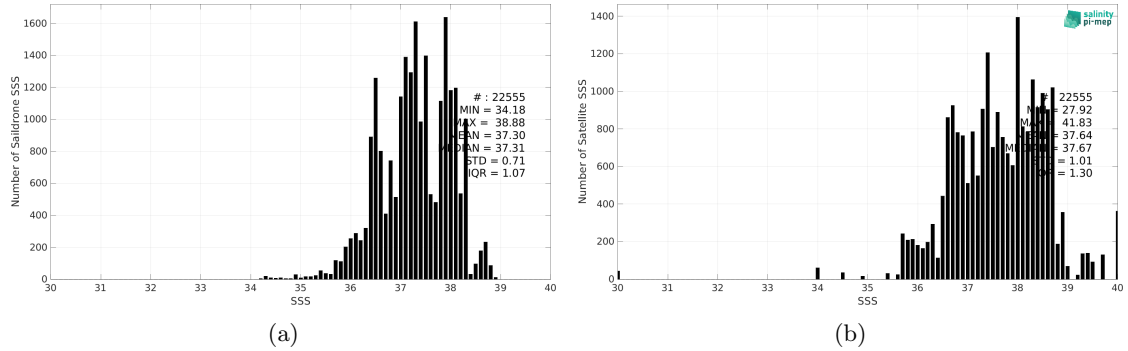
Figure 2: Histograms of SSS from Saildrone (a) and SMOS SSS L3 v2 - 9-Days (BEC) (b) considering all match-up pairs per bins of 0.1 over the Mediterranean Sea Pi-MEP region and for the full satellite product period.
