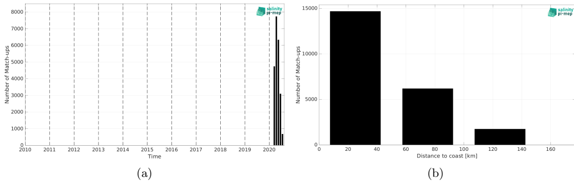
Figure 1: Number of match-ups between Saildrone and SMOS SSS L3 v2 - 9-Days (BEC) SSS as a function of time (a) and as function of the distance to coast (b) over the Mediterranean Sea Pi-MEP region and for the full satellite product period.
