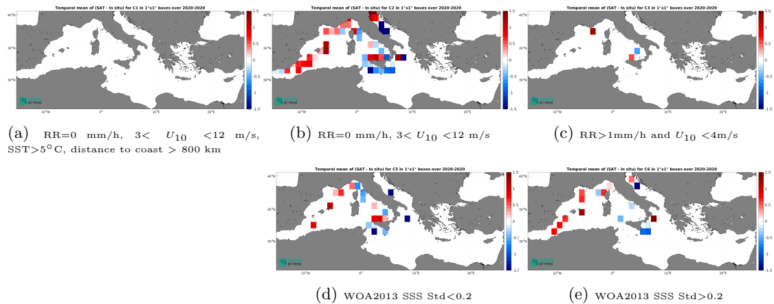
Figure 12: Temporal mean gridded over spatial boxes of size 1^\circ \times 1^\circ of \Delta\text{SSS} (SMOS SSS L3 v2 - 9-Days (BEC) - Saildrone) for 5 different subdatasets corresponding to:RR=0 mm/h, 3 < U_{10} < 12 m/s, SST >5^\circ\text{C} , distance to coast > 800 km (a), RR=0 mm/h, 3 < U_{10} < 12 m/s (b), RR >1 mm/h and U_{10} < 4 m/s (c), WOA2013 SSS Std <0.2 (d), WOA2013 SSS Std >0.2 (e).
