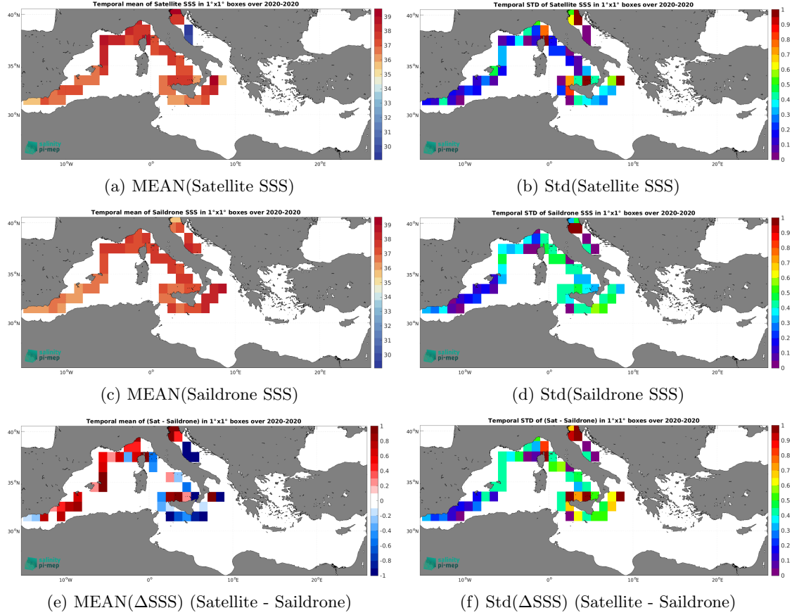
Figure 6: Temporal mean (left) and Std (right) of SSS from SMOS SSS L3 v2 - 9-Days (BEC) (top), Saildrone (middle), and of \Delta SSS (Satellite - Saildrone). Only match-up pairs are used to generate these maps.
