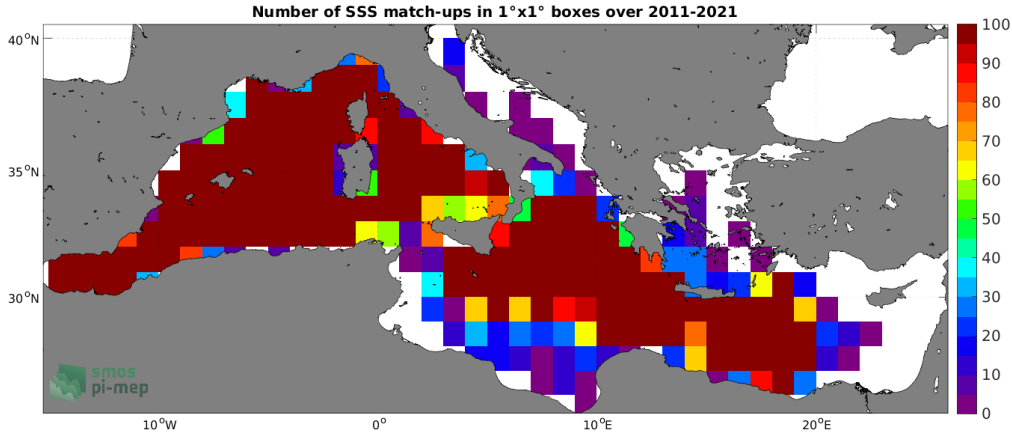
Figure 4: Number of SSS match-ups between Argo SSS and the SMOS SSS L3 v2 - 9-Days (BEC) SSS product for the Mediterranean Sea Pi-MEP region over 1^\circ \times 1^\circ boxes and for the full satellite product period.
