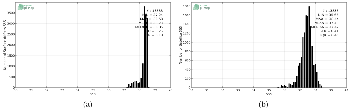
Figure 2: Histograms of SSS from Surface drifters (a) and SMOS-L3-BEC-OA-V1-9DAYS-0.25DEG (b) considering all match-up pairs per bins of 0.1 over the Mediterranean Sea Pi-MEP region and for the full satellite product period.
