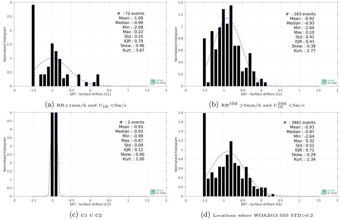
Figure 12: Normalized histogram of \Delta SSS (SMOS-L3-BEC-OA-V1-9DAYS-0.25DEG - Surface drifters) for 6 different subdatasets corresponding to: RR > 1mm/h and U_{10} < 5 m/s (a), RR^{10d} > 5 mm/h and U_{10}^{10d} < 5 m/s (b), C1 U C2 (c), Locations where WOA2013 SSS STD > 0.2 (d).
