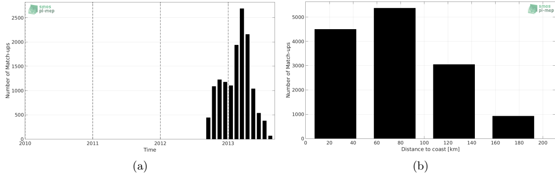
Figure 1: Number of match-ups between Surface drifters and SMOS-L3-BEC-OA-V1-9DAYS-0.25DEG SSS as a function of time (a) and as function of the distance to coast (b) over the Mediterranean Sea Pi-MEP region and for the full satellite product period.
