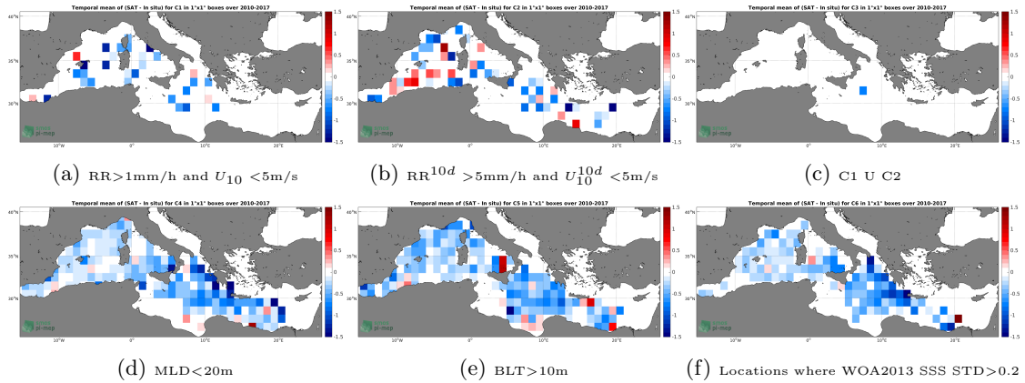
Figure 12: Temporal mean gridded over spatial boxes of size 1°x1° of \Delta SSS (SMOS-L3-BEC-OA-V1-9DAYS-0.25DEG - Argo) for 6 different subdatasets corresponding to:RR>1mm/h and U_{10} < 5m/s (a), RR^{10d} > 5mm/h and U_{10}^{10d} < 5m/s (b), C1 U C2 (c),MLD<20m (d),BLT>10m (e),Locations where WOA2013 SSS STD>0.2 (f).
