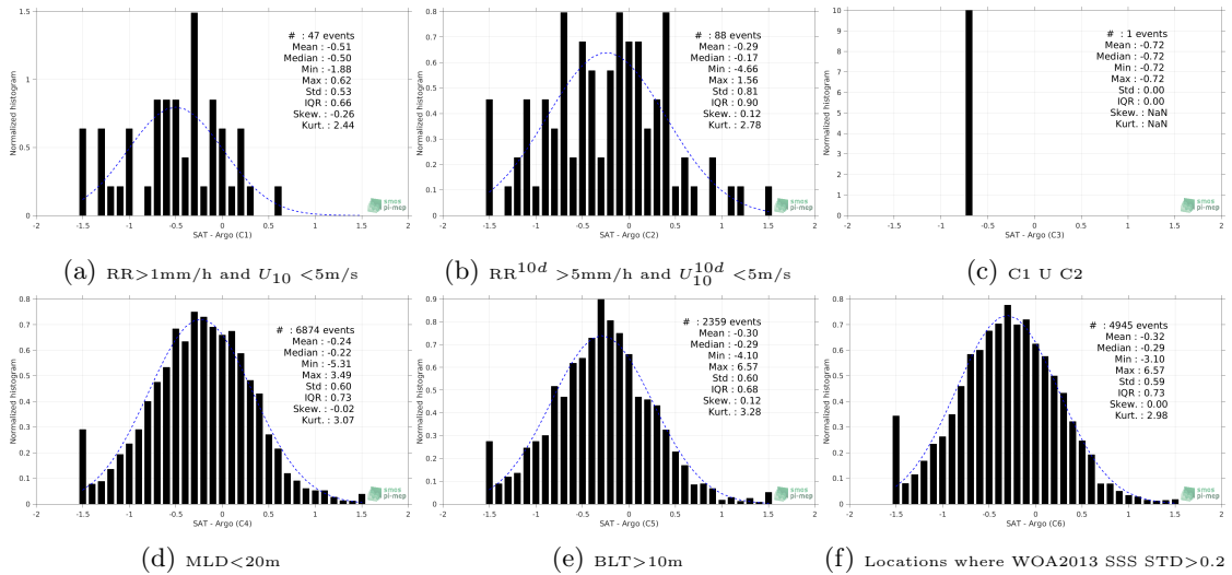
Figure 13: Normalized histogram of \Delta SSS (SMOS-L3-BEC-OA-V1-9DAYS-0.25DEG - Argo) for 6 different subdatasets corresponding to: RR>1mm/h and U_{10} < 5m/s (a), RR^{10d} > 5mm/h and U_{10}^{10d} < 5m/s (b), C1 U C2 (c),MLD<20m (d),BLT>10m (e),Locations where WOA2013 SSS STD>0.2 (f).
