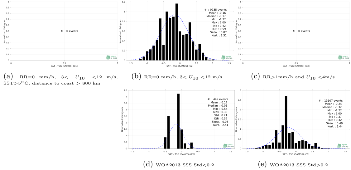
Figure 13: Normalized histogram of \Delta SSS (SMOS SSS L3 MED-ATL-OA v2 - 9 Days (BEC) - TSG (SAMOS)) for 5 different subdatasets corresponding to: RR=0 mm/h, 3 < U_{10} < 12 m/s, SST > 5°C, distance to coast > 800 km (a), RR=0 mm/h, 3 < U_{10} < 12 m/s (b), RR > 1mm/h and U_{10} < 4 m/s (c), WOA2013 SSS Std < 0.2 (d), WOA2013 SSS Std > 0.2 (e).
