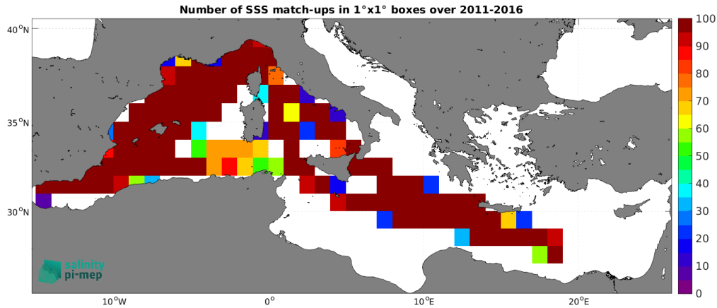
Figure 5: Number of SSS match-ups between TSG (LEGOS-DM) SSS and the SMOS SSS L3 MED-ATL-OA v2 - 9 Days (BEC) SSS product for the Mediterranean Sea Pi-MEP region over 1^\circ \times 1^\circ boxes and for the full satellite product period.
