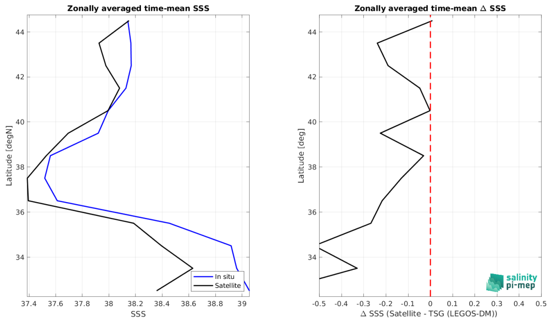
Figure 9: Left panel: Zonal mean SSS from SMOS SSS L3 MED-ATL-OA v2 - 9 Days (BEC) satellite product (black) and from TSG (LEGOS-DM) (blue). Right panel: Zonal mean of \Delta SSS (Satellite - TSG (LEGOS-DM)) for all the collected Pi-MEP match-up pairs estimated over the full satellite product period.
