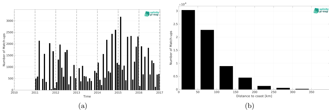
Figure 2: Number of match-ups between TSG (LEGOS-DM) and SMOS SSS L3 MED-ATL-OA v2 - 9 Days (BEC) SSS as a function of time (a) and as function of the distance to coast (b) over the Mediterranean Sea Pi-MEP region and for the full satellite product period.
