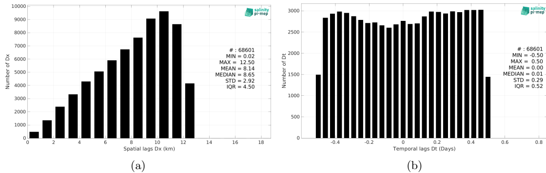
Figure 6: Histograms of the spatial (a) and temporal (b) lags between the location/time of the TSG (LEGOS-DM) measurement and the date of the corresponding SMOS SSS L3 MED-ATL-OA v2 - 9 Days (BEC) SSS pixel.
