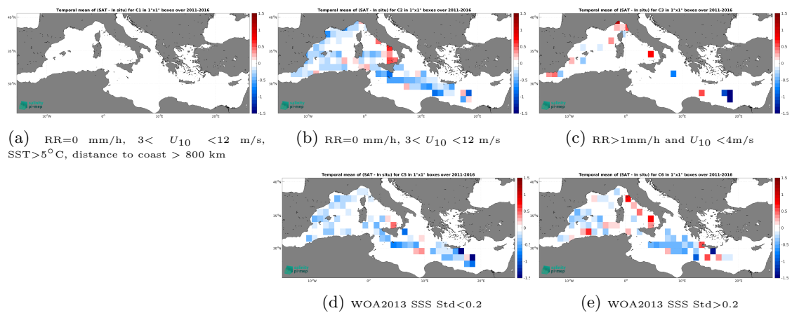
Figure 14: Temporal mean gridded over spatial boxes of size 1^\circ \times 1^\circ of \Delta\text{SSS} (SMOS SSS L3 MED-ATL-OA v2 - 9 Days (BEC) - TSG (LEGOS-DM)) for 5 different subdatasets corresponding to:RR=0 mm/h, 3 < U_{10} < 12 m/s, SST>5°C, distance to coast > 800 km (a), RR=0 mm/h, 3 < U_{10} < 12 m/s (b), RR>1mm/h and U_{10} < 4 m/s (c), WOA2013 SSS Std<0.2 (d), WOA2013 SSS Std>0.2 (e).
