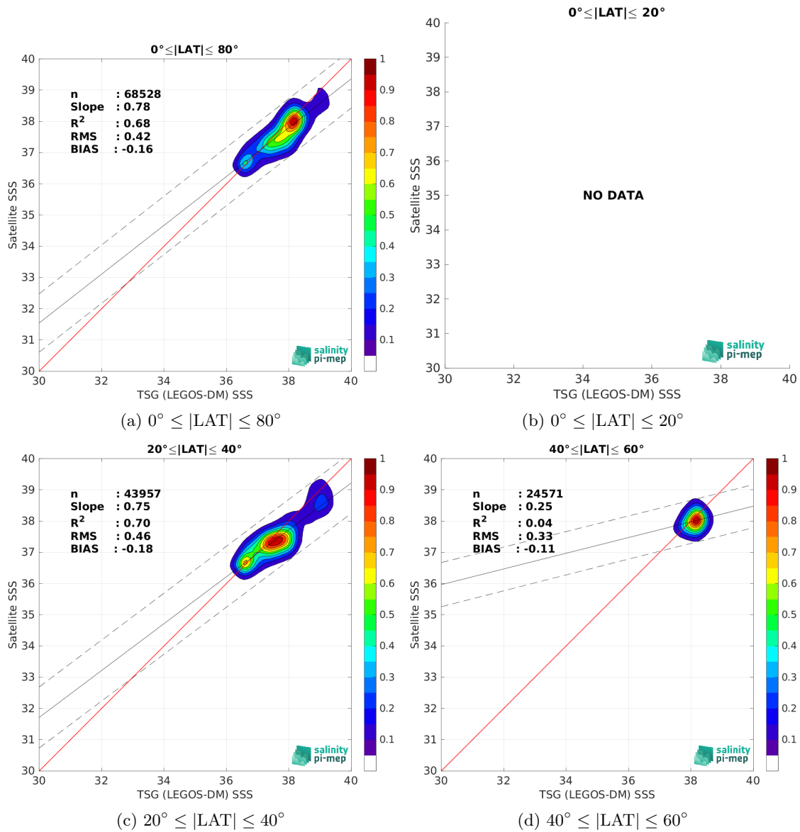
Figure 10: Contour maps of the concentration of SMOS SSS L3 MED-ATL-OA v2 - 9 Days (BEC) SSS (y-axis) versus TSG (LEGOS-DM) SSS (x-axis) at match-up pairs for different latitude bands. For each plot, the red line shows x=y . The black thin and dashed lines indicate a linear fit through the data cloud and the \pm 95\% confidence levels, respectively. The number match-up pairs n , the slope and R^2 coefficient of the linear fit, the root mean square (RMS) and the mean bias between satellite and in situ data are indicated for each latitude band in each plots.
