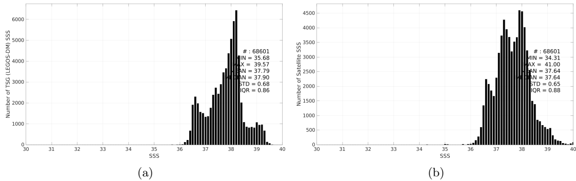
Figure 3: Histograms of SSS from TSG (LEGOS-DM) (a) and SMOS SSS L3 MED-ATL-OA v2 - 9 Days (BEC) (b) considering all match-up pairs per bins of 0.1 over the Mediterranean Sea Pi-MEP region and for the full satellite product period.
