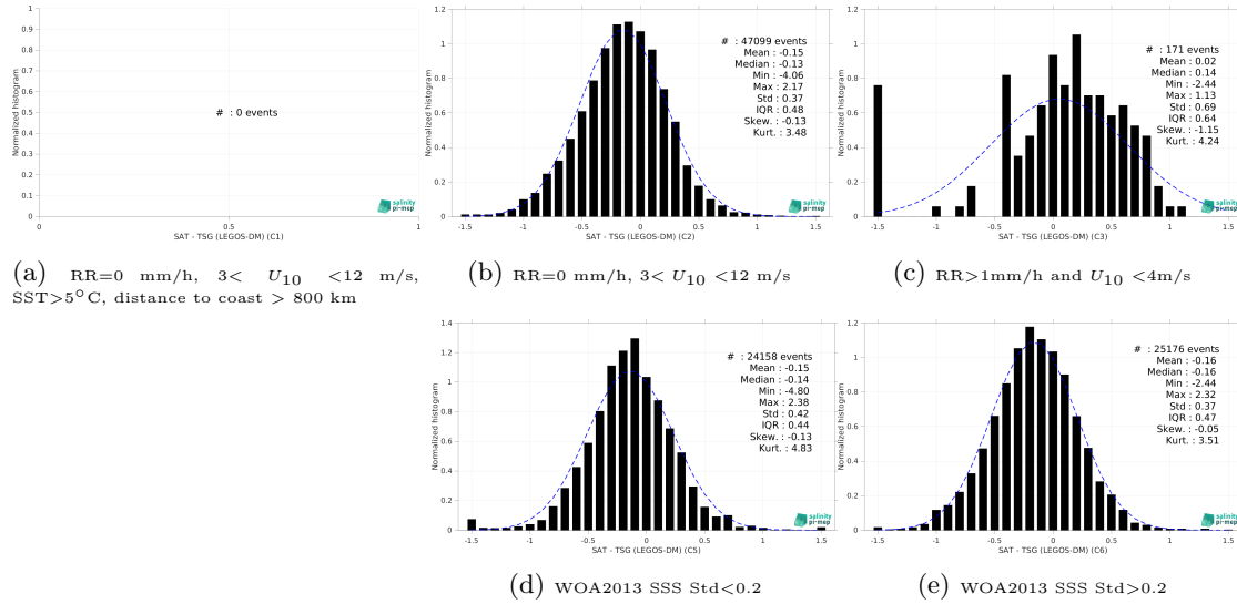
Figure 15: Normalized histogram of \Delta SSS (SMOS SSS L3 MED-ATL-OA v2 - 9 Days (BEC) - TSG (LEGOS-DM)) for 5 different subdatasets corresponding to: RR=0 mm/h, 3 < U_{10} < 12 m/s, SST > 5°C, distance to coast > 800 km (a), RR=0 mm/h, 3 < U_{10} < 12 m/s (b), RR > 1mm/h and U_{10} < 4 m/s (c), WOA2013 SSS Std < 0.2 (d), WOA2013 SSS Std > 0.2 (e).
