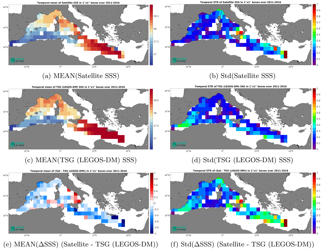
Figure 7: Temporal mean (left) and Std (right) of SSS from SMOS SSS L3 MED-ATL-OA v2 - 9 Days (BEC) (top), TSG (LEGOS-DM) (middle), and of \Delta\text{SSS} (Satellite - TSG (LEGOS-DM)). Only match-up pairs are used to generate these maps.
