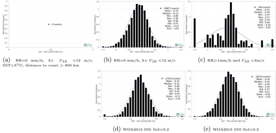
Figure 13: Normalized histogram of \Delta SSS (SMOS SSS L3 MED-ATL-OA v2 - 9 Days (BEC) - TSG (LEGOS-DM)) for 5 different subdatasets corresponding to: RR=0 mm/h, 3 < U_{10} < 12 m/s, SST > 5°C, distance to coast > 800 km (a), RR=0 mm/h, 3 < U_{10} < 12 m/s (b), RR > 1mm/h and U_{10} < 4 m/s (c), WOA2013 SSS Std < 0.2 (d), WOA2013 SSS Std > 0.2 (e).
